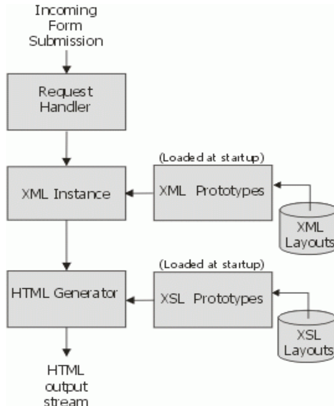
Figure 1 iCS 5.0 XML Processing
