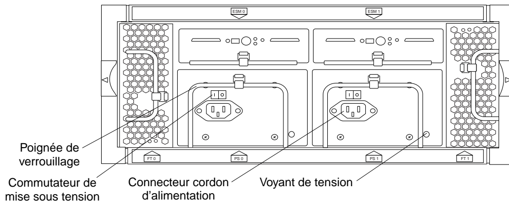
FIGURE 1-10 Alimentations
