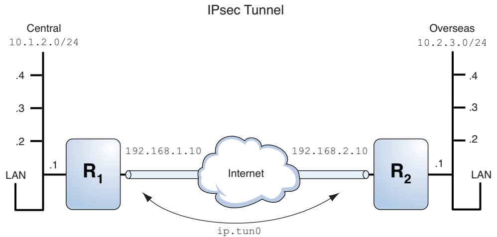
FIGURE 20-1 IPsec Tunnel Diagram
