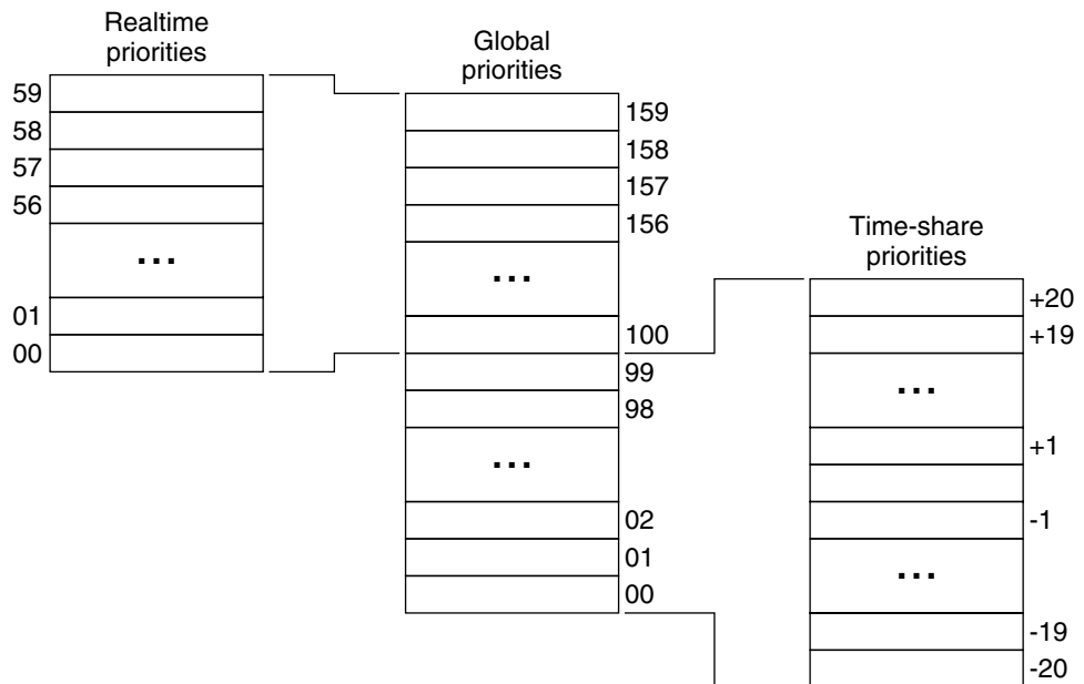
FIGURE 12-5 Kernel Dispatch Queue
