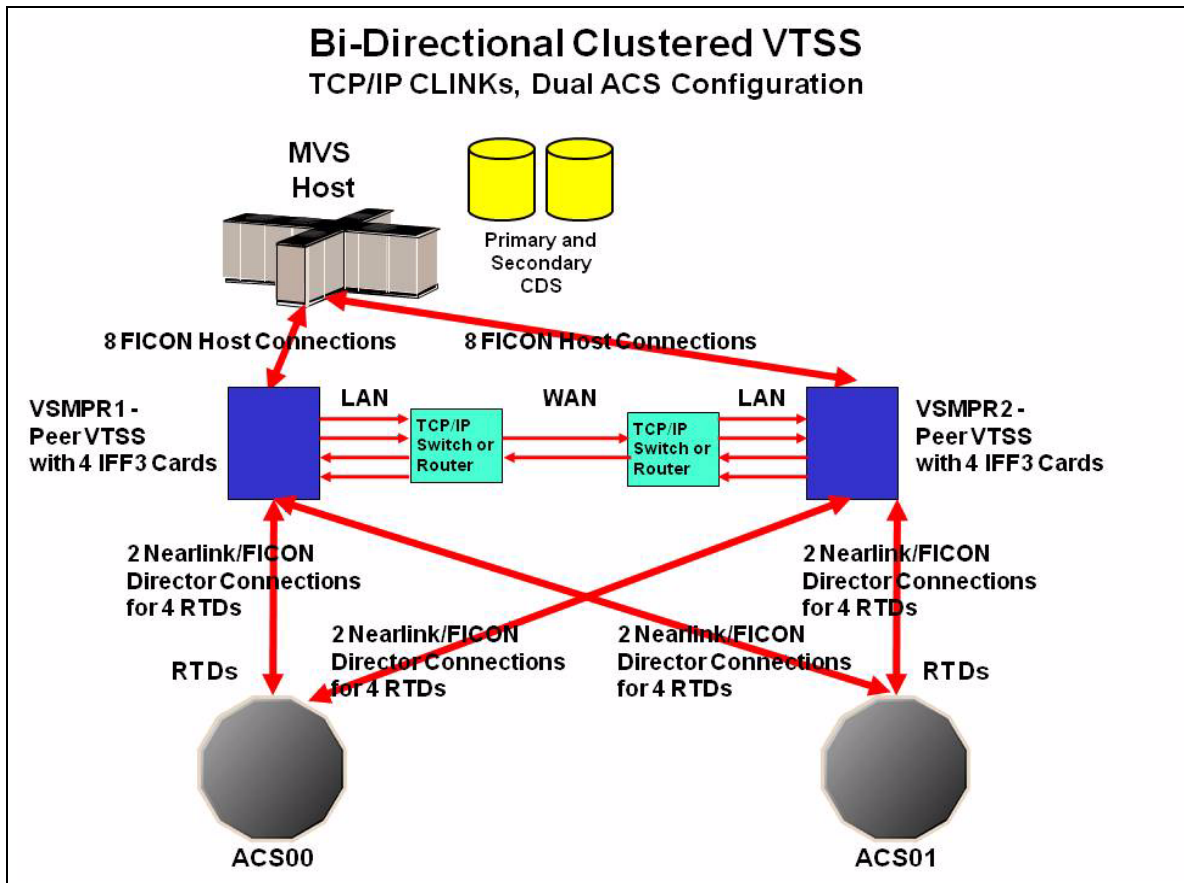
Figure 28. Clustered VTSS with TCP/IP IP CLINKs
