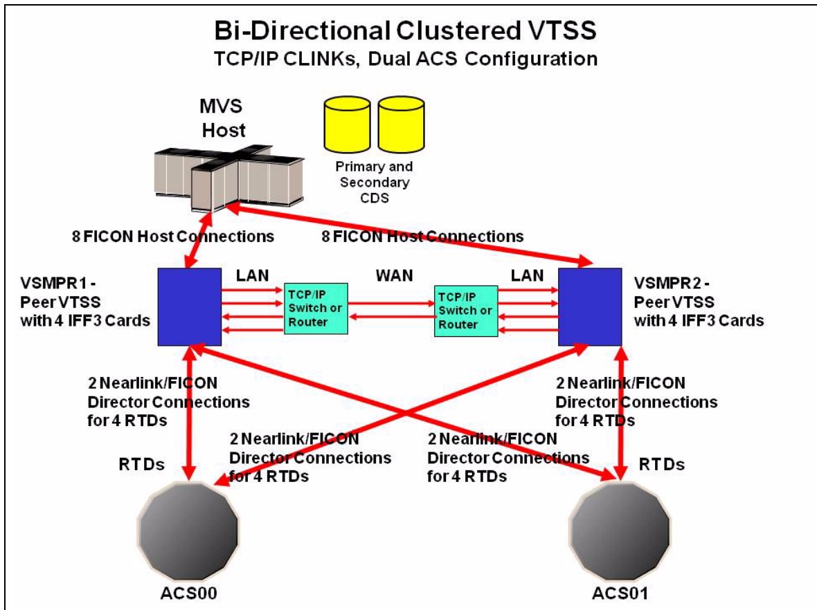
Figure 24. The TCP/IP Environment with IFF3 Cards for TCP/IP CLINKs
