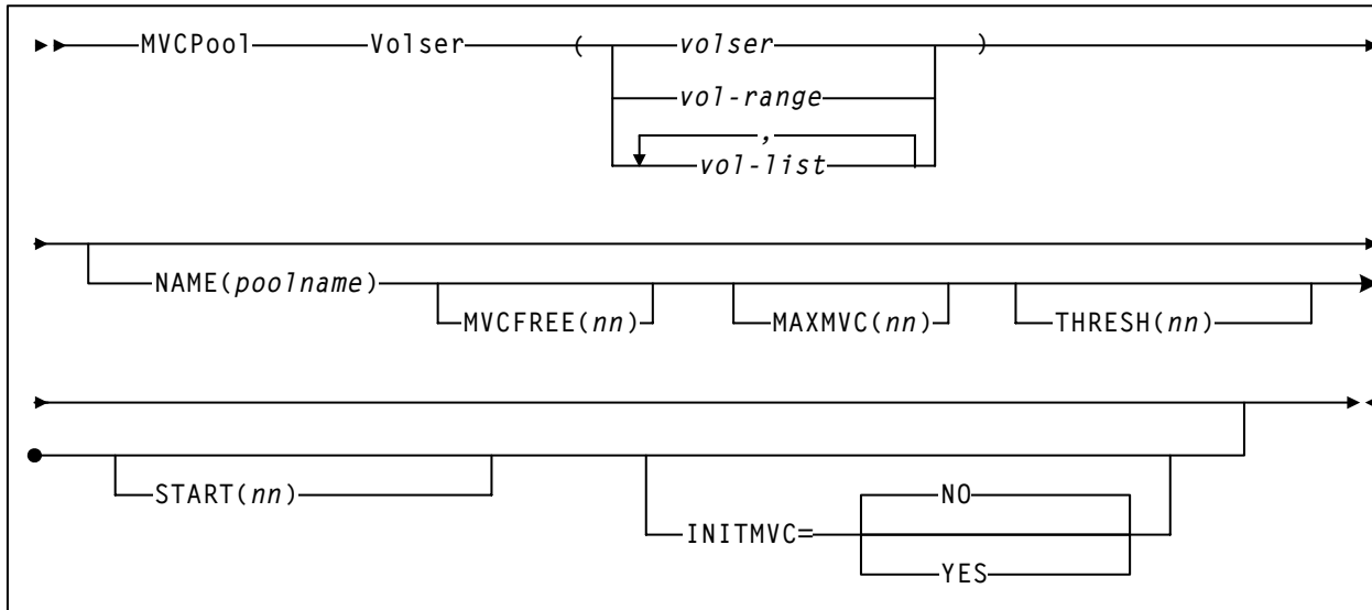
Figure 11. MVCPool Control Statement Syntax
