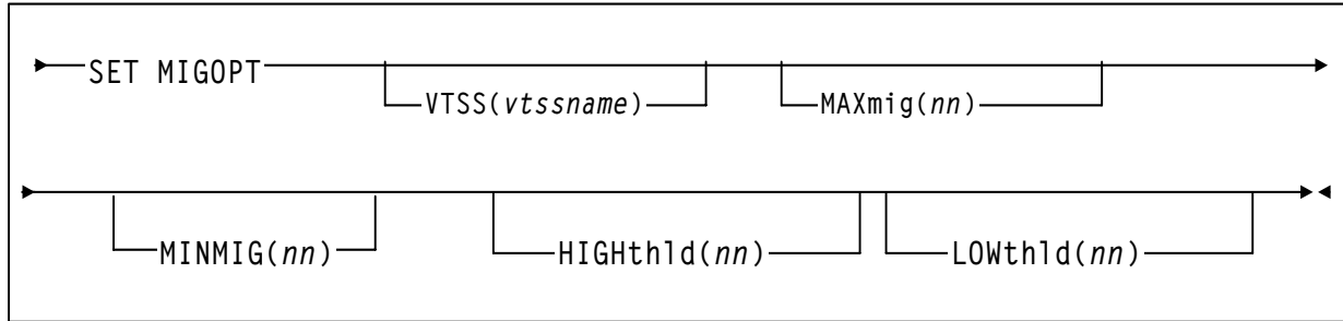
Figure 102. SET MIGOPT syntax
