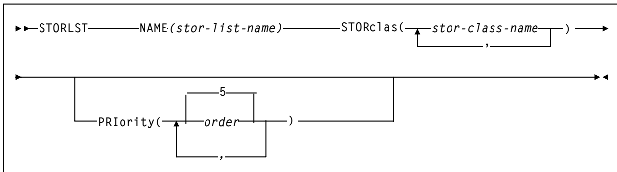
Figure 13. STORLST Control Statement Syntax
