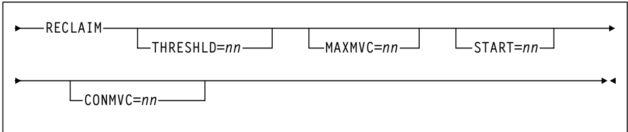
Figure 8. RECLAIM statement syntax
