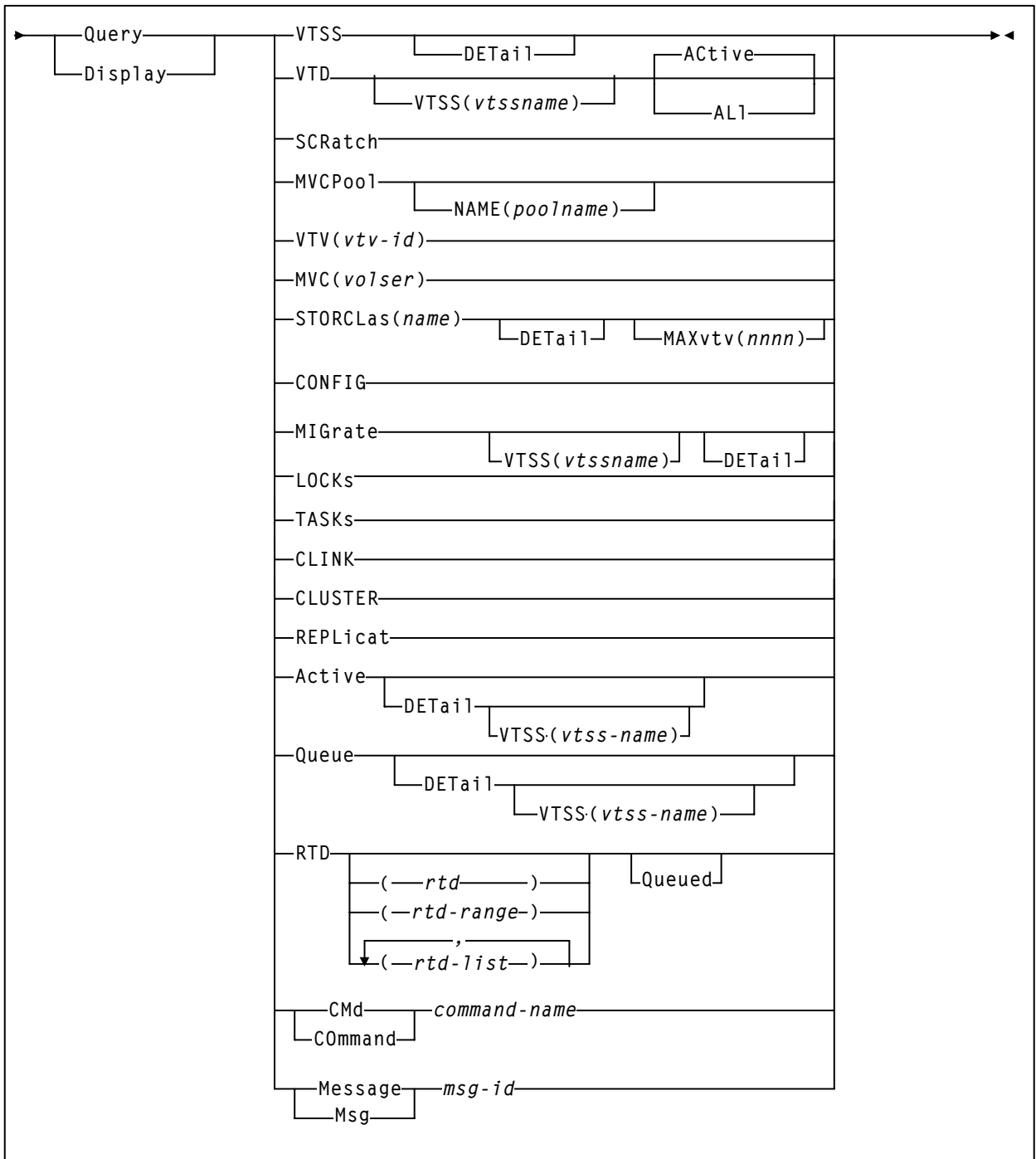
Figure 31. Query Display syntax
