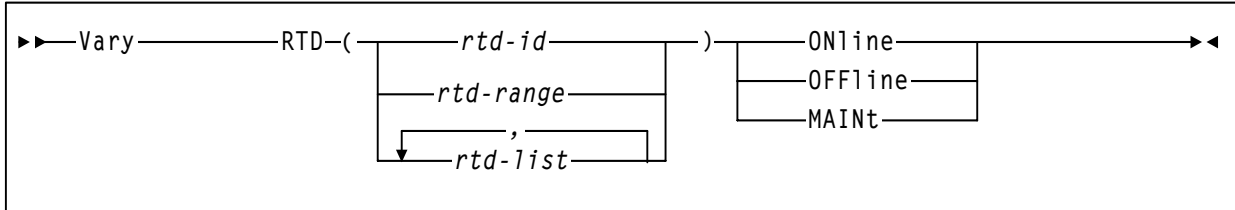
Figure 109. Vary RTD syntax
