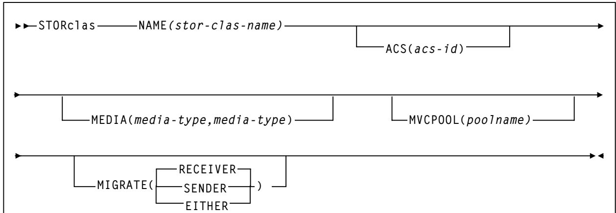
Figure 12. STORCLAS Control Statement Syntax
