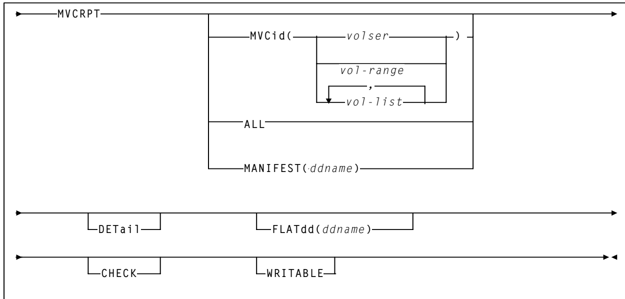
Figure 84. MVCRPT syntax
