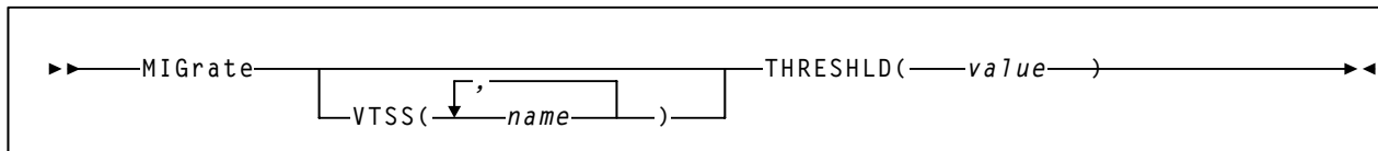
Figure 70. MIGRATE utility syntax - Format 2
