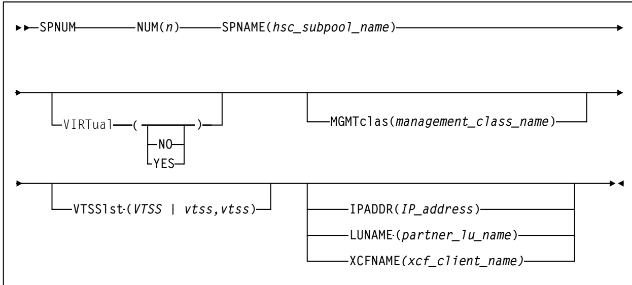
Figure 1. SPNUM Statement Syntax
