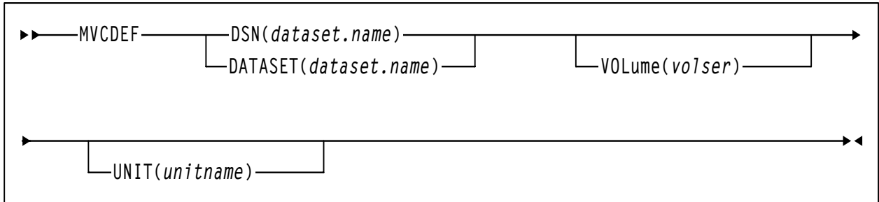
Figure 73. VT MVCDEF command syntax
