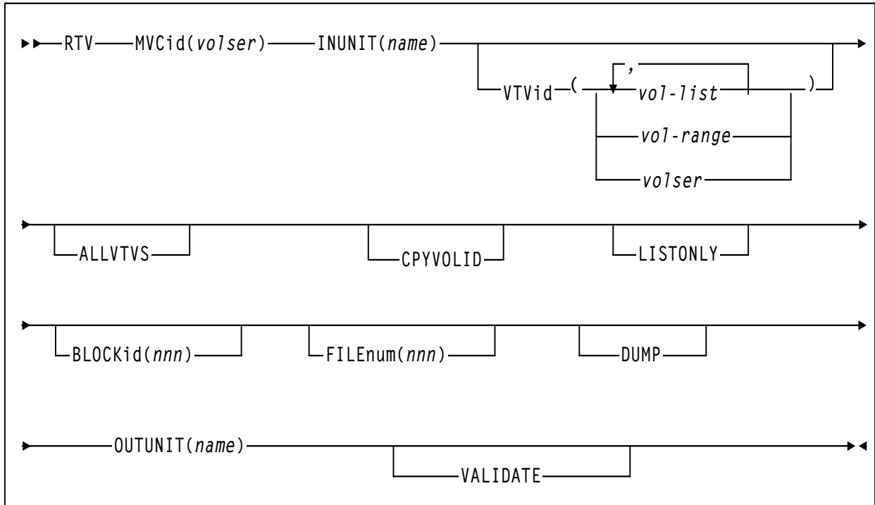
Figure 96. RTV utility syntax
