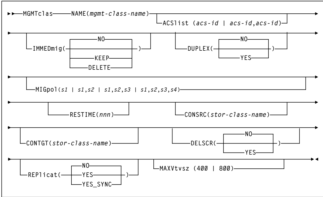
Figure 9. MGMTclas Control Statement Syntax - Advanced Management Feature
