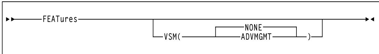
Figure 2. FEATures Control Statement
