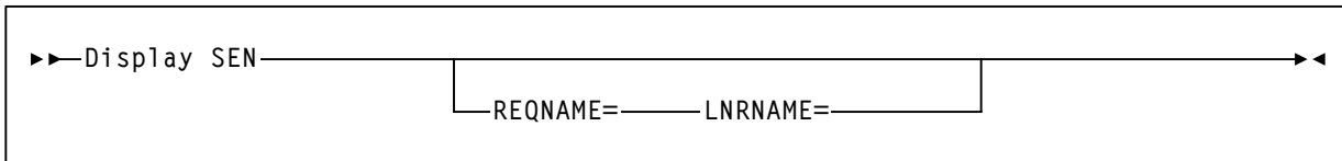
Figure 3. Display SEN Syntax
