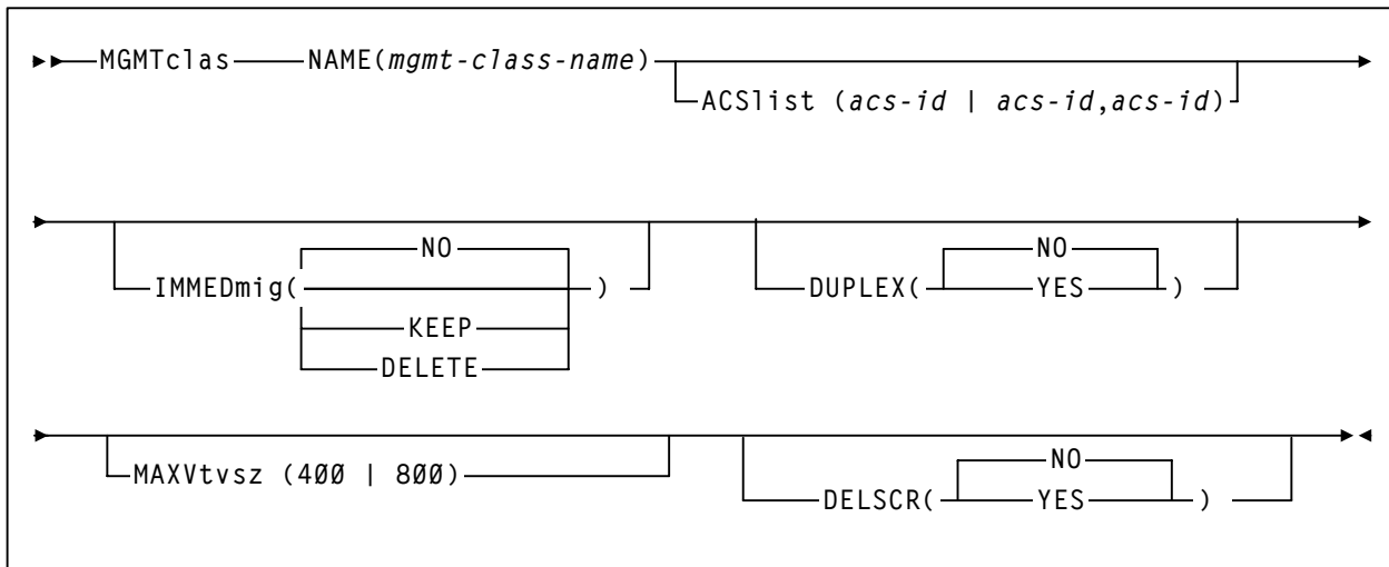
Figure 8. MGMTclas Control Statement Syntax - Basic Management Feature
