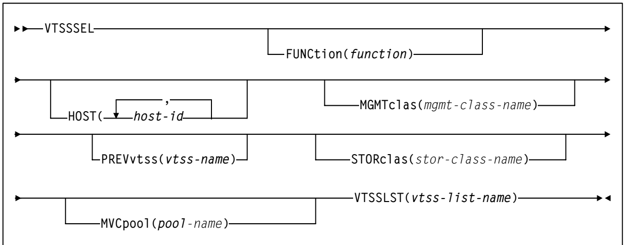
Figure 17. VTSSSEL Control Statement Syntax
