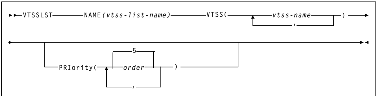
Figure 16. VTSSLST Control Statement Syntax
