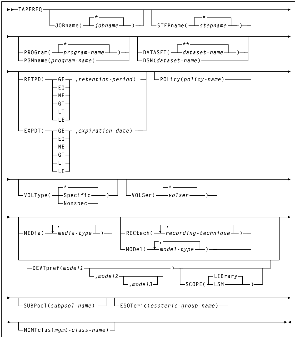
Figure 1. TAPEREQ Control Statement Syntax
