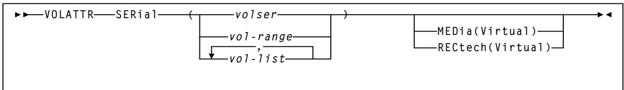
Figure 15. VOLATTR Control Statement Syntax
