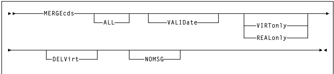
Figure 3. MERGEcds Utility Syntax
