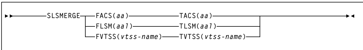
Figure 4. SLSMERGE DD Statement Syntax
