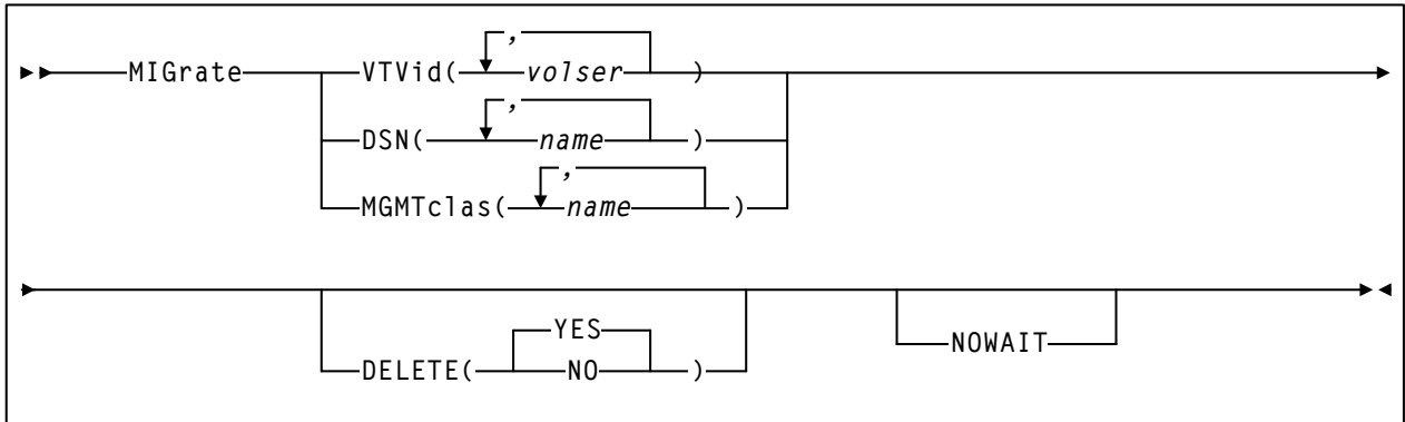
Figure 69. MIGRATE utility syntax - Format 1
