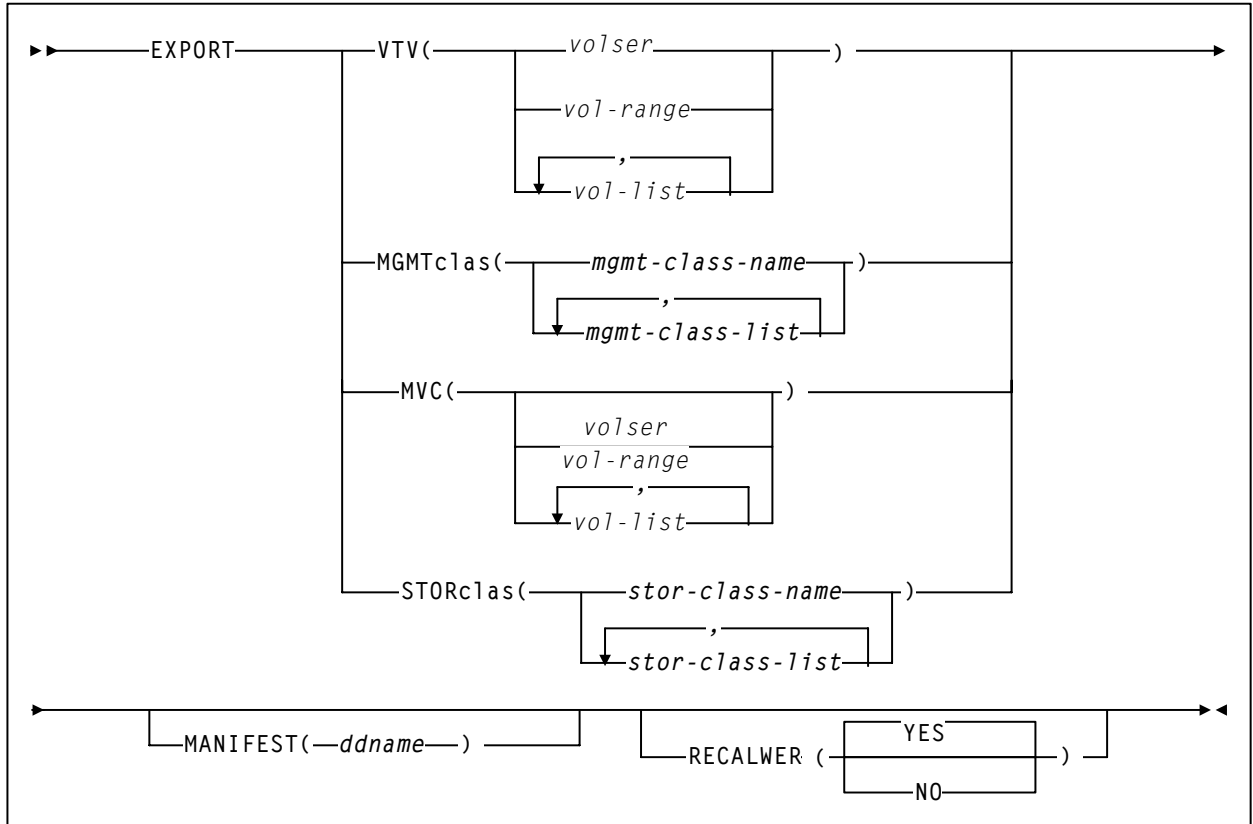
Figure 55. EXPORT utility syntax
