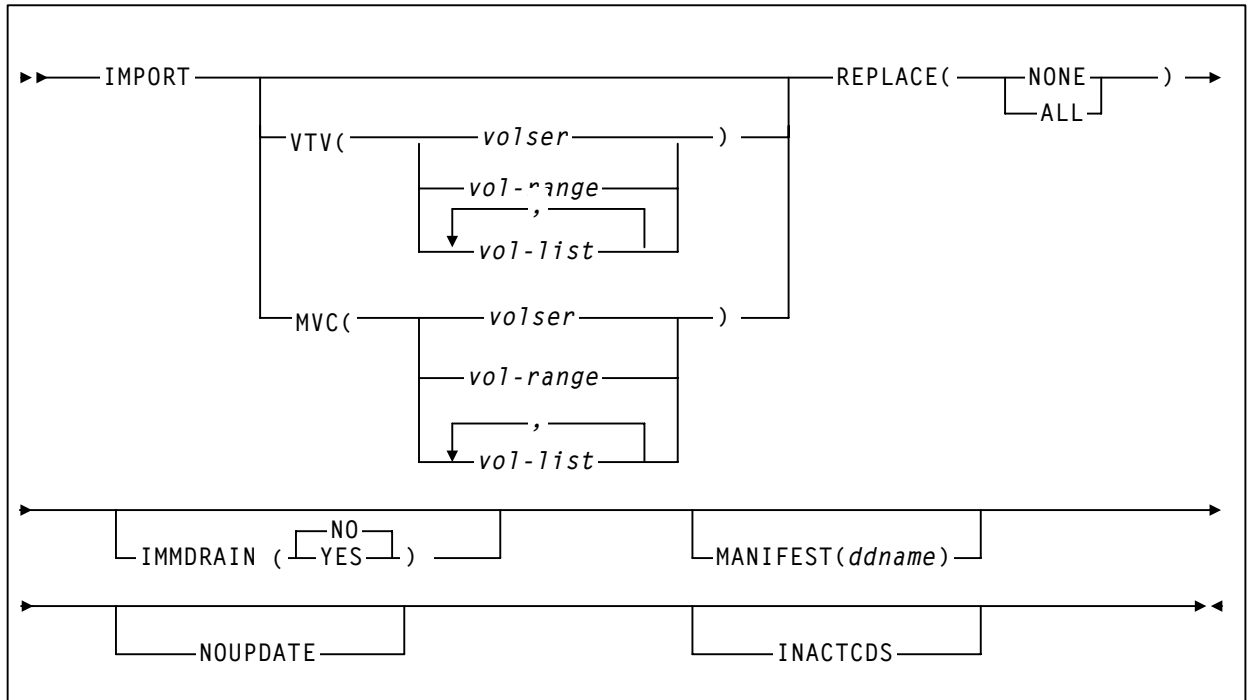
Figure 58. IMPORT utility syntax
