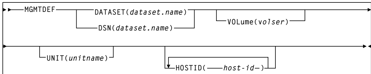
Figure 10. MGMTDEF Command
