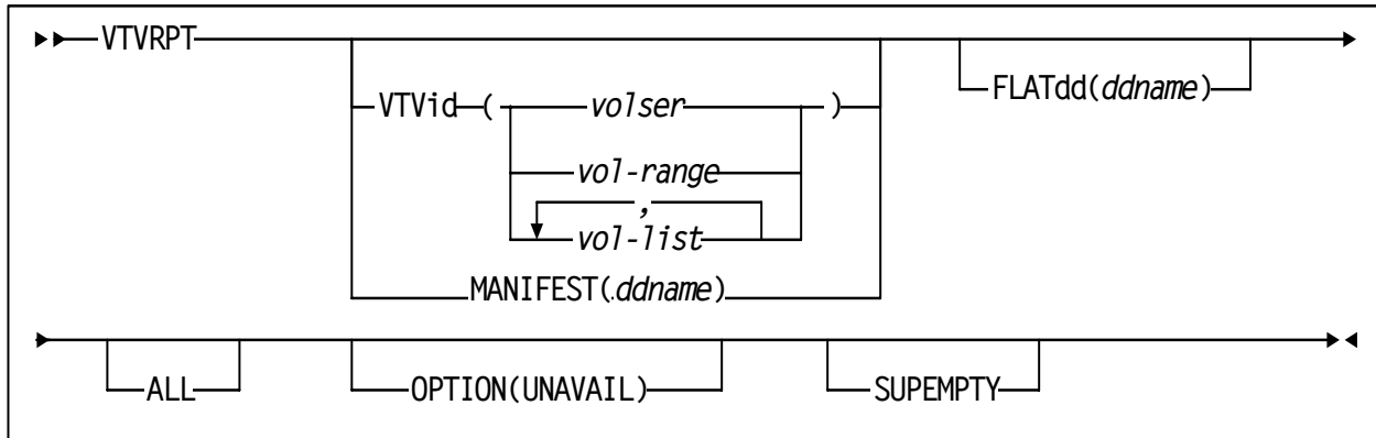
Figure 116. VTVRPT syntax
