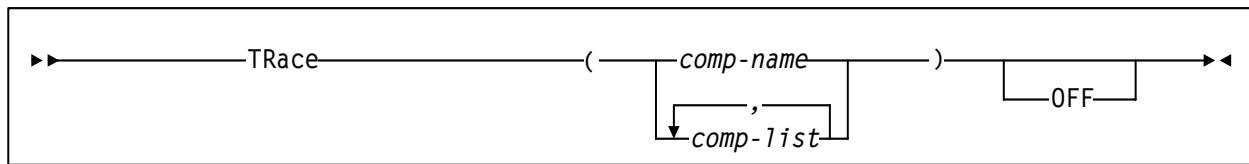
Figure 105. TRace syntax
