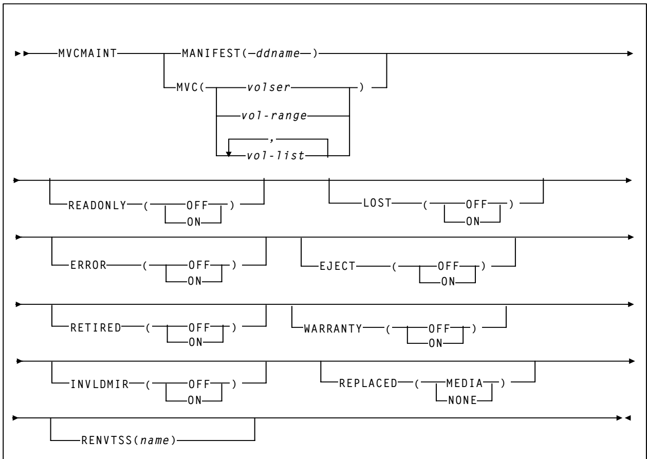
Figure 76. MVCMaint syntax
