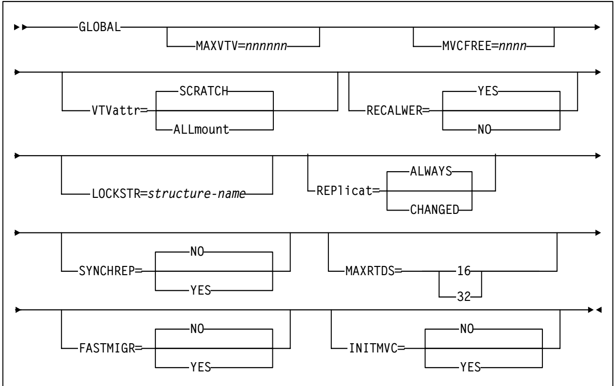
Figure 7. GLOBAL statement syntax
