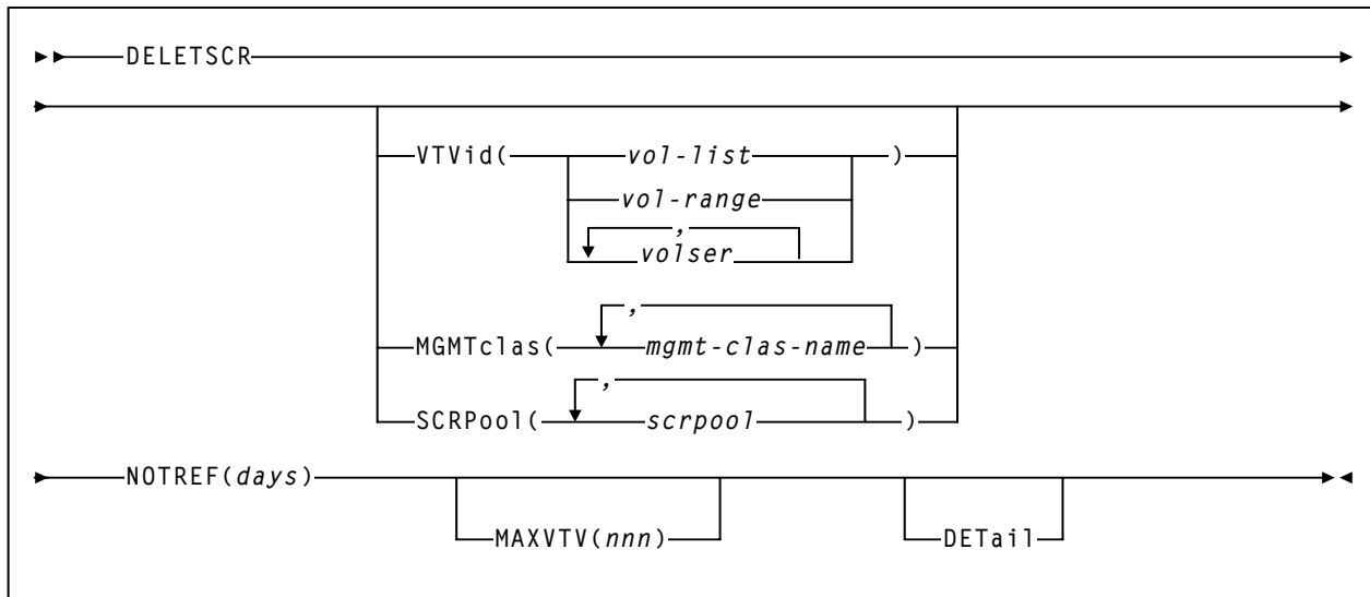
Figure 29. DELETSCR syntax
