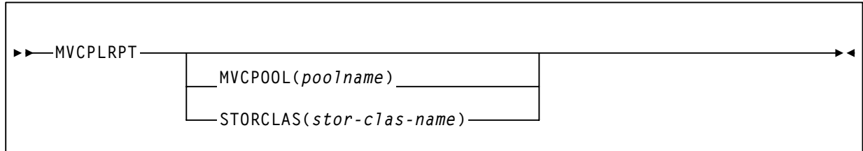
Figure 80. MVCPLRPT syntax
