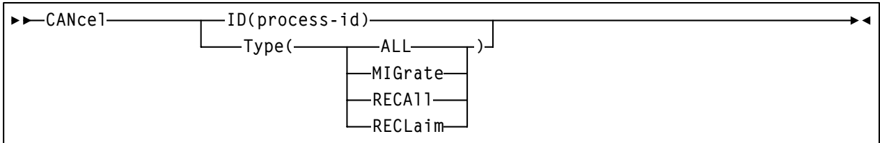
Figure 4. CANce1 syntax
