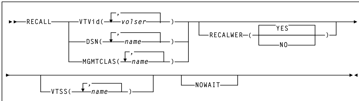
Figure 91. RECALL syntax
