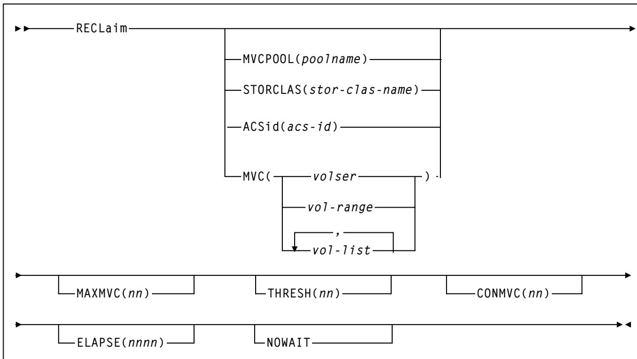
Figure 93. RECLAIM syntax
