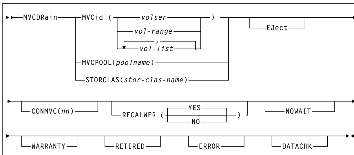
Figure 74. MVCDRAIN syntax
