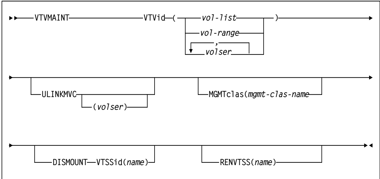
Figure 113. VTVMaint syntax
