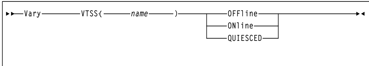
Figure 111. Vary VTSS syntax
