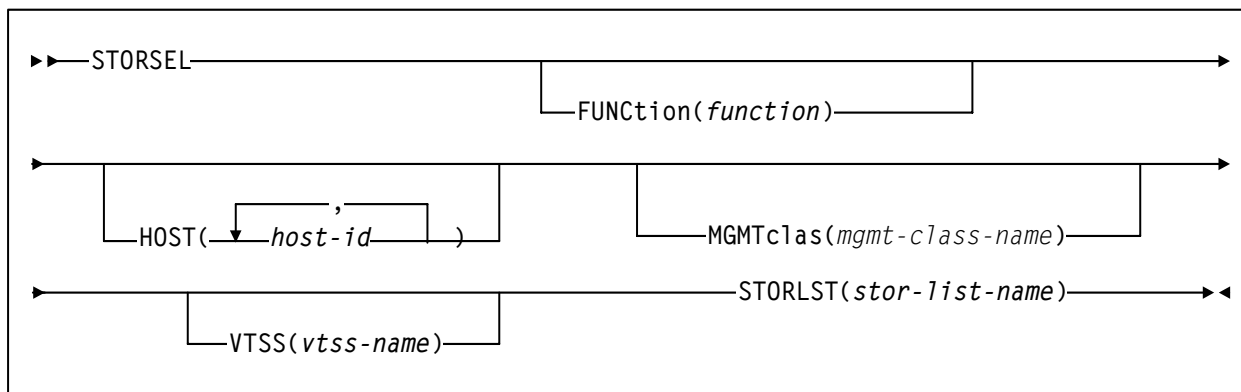
Figure 14. STORSEL Control Statement Syntax
