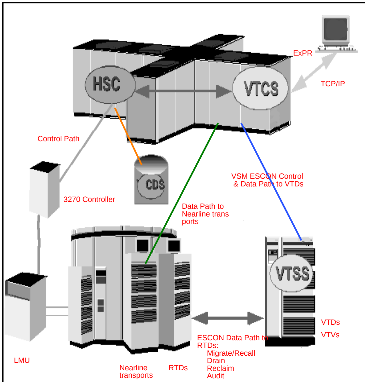
Figure 1. Simple VSM Configuration
