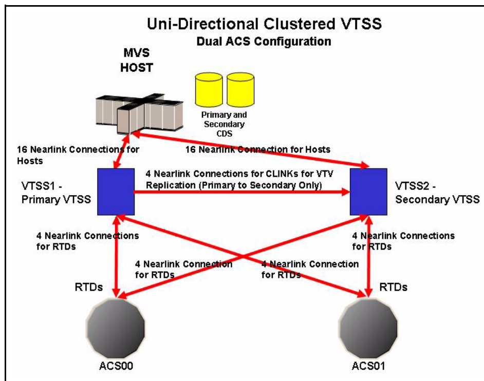
Figure 8. Uni-Directional Clustered VTSS Dual ACS Configuration
