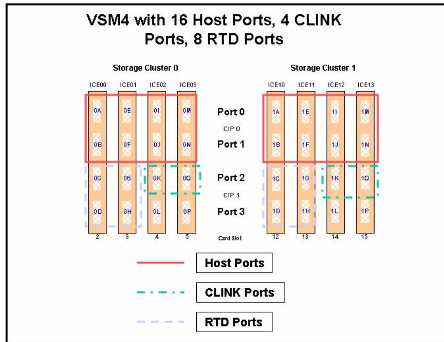
Figure 7. VSM4 with 16 Host Ports, 4 CLINK Ports, 12 RTD Ports (All ESCON)
