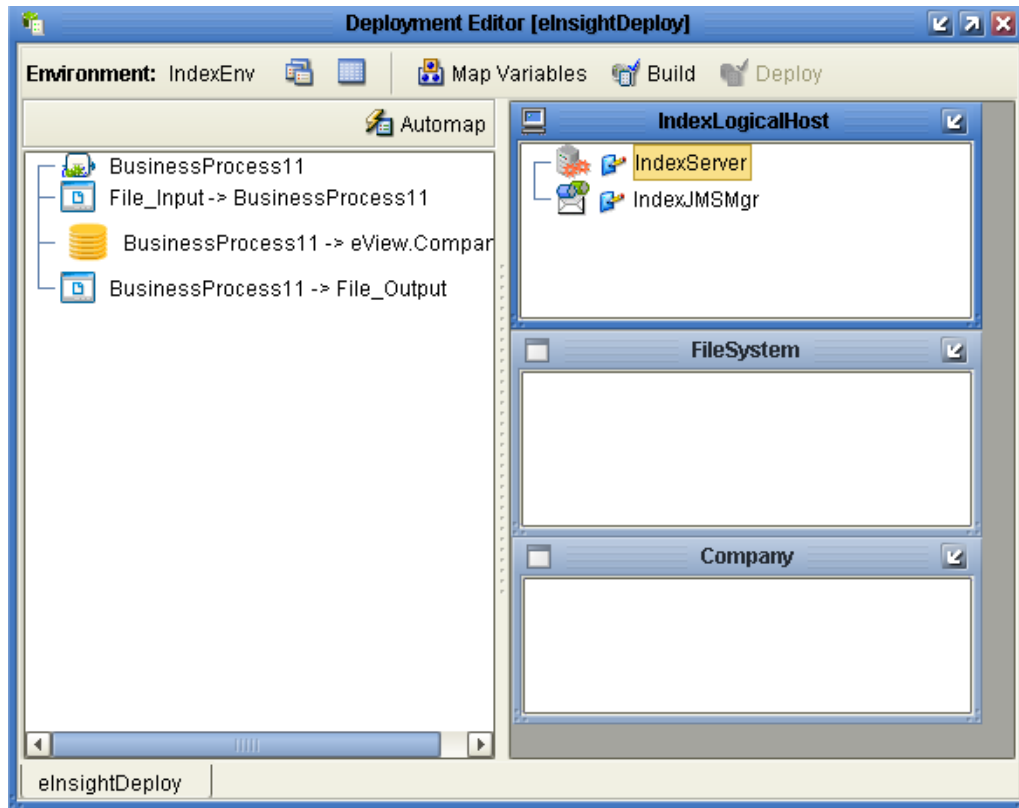
Figure 64 Deployment Editor Window
