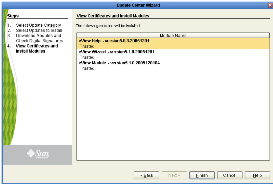
Figure 13 Update Center Wizard - View Certificates and Install Modules
