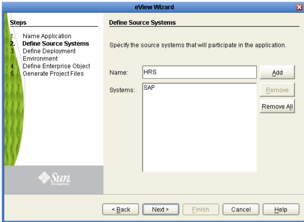
Figure 18 eView Wizard - Define Source Systems
