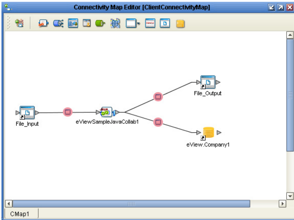
Figure 38 Collaboration Client Connectivity Map With Connections
