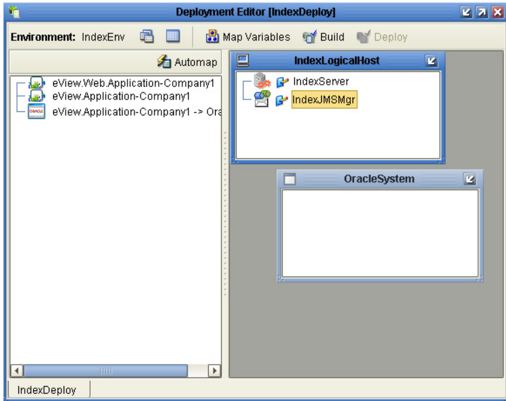
Figure 57 Deployment Editor - Server Project
