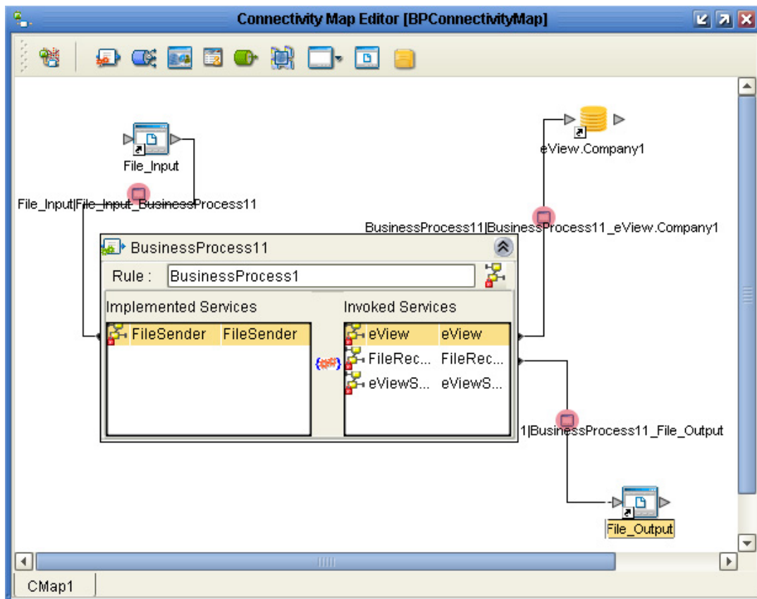
Figure 46 Service Binding Dialog Connections, eInsight BPM
