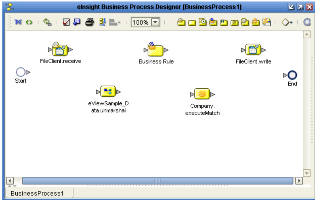
Figure 42 eInsight Business Process with eView Studio Activity
