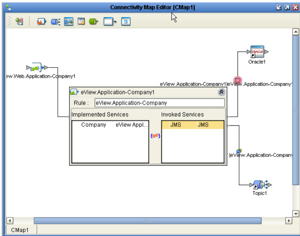
Figure 32 Server Connectivity Map with Connections
