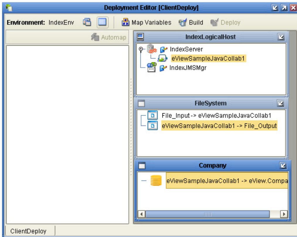
Figure 62 Mapped Client Components in the Deployment Editor
