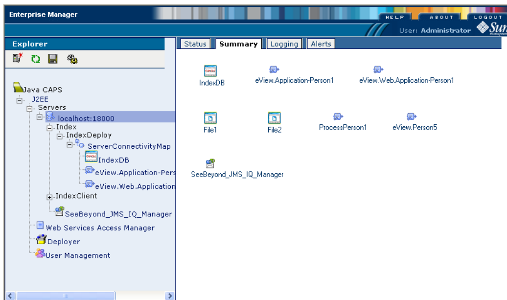
Figure 67 Monitoring eView Studio Project Components
