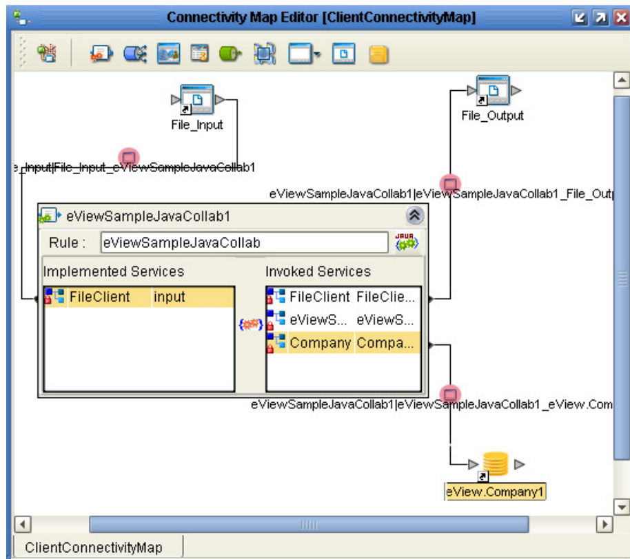
Figure 37 Collaboration Client - Service Binding Dialog Connections
