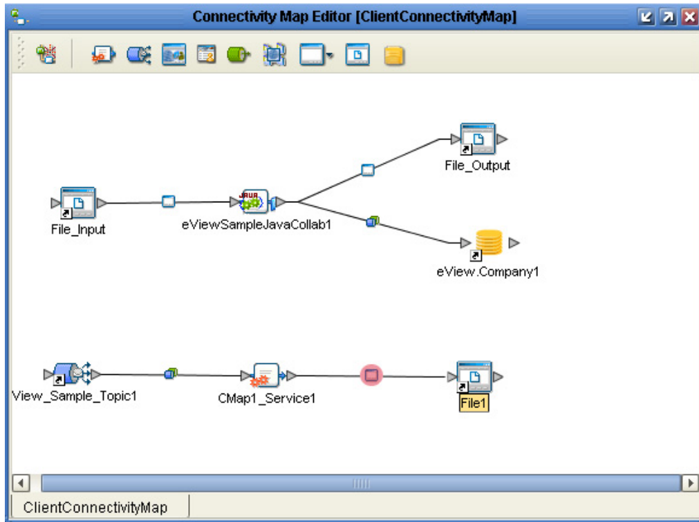
Figure 40 Collaboration Client Connectivity Map with JMS Topic Connections
