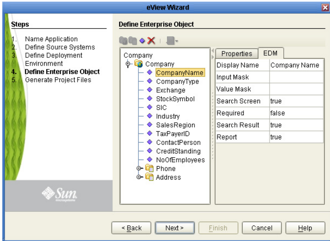
Figure 26 Field EDM Page
