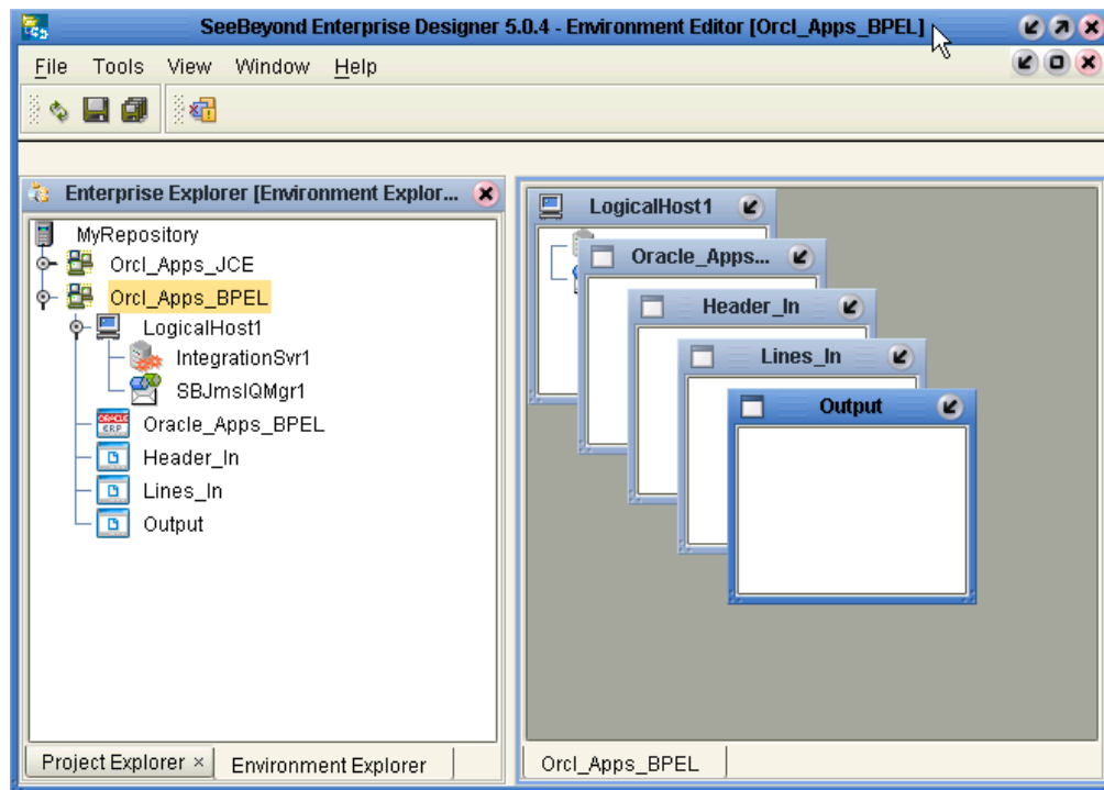
Figure 31 Orcl_Apps_BPEL Environment
