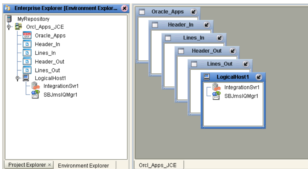
Figure 20 Orcl_Apps_JCD Environment
