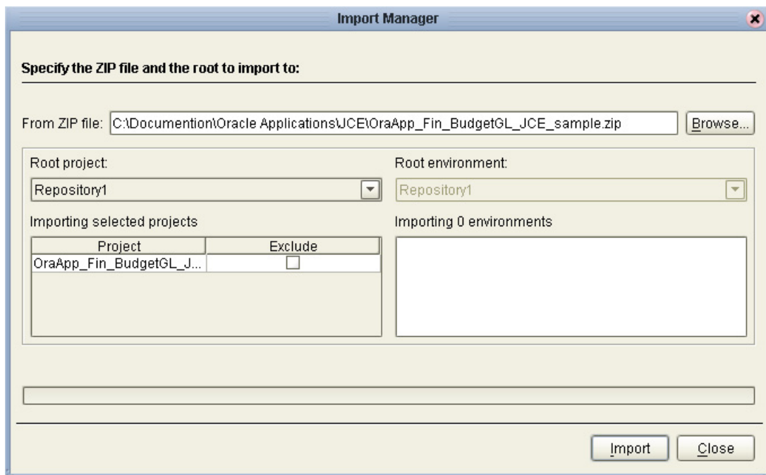
Figure 34 Import Manager
