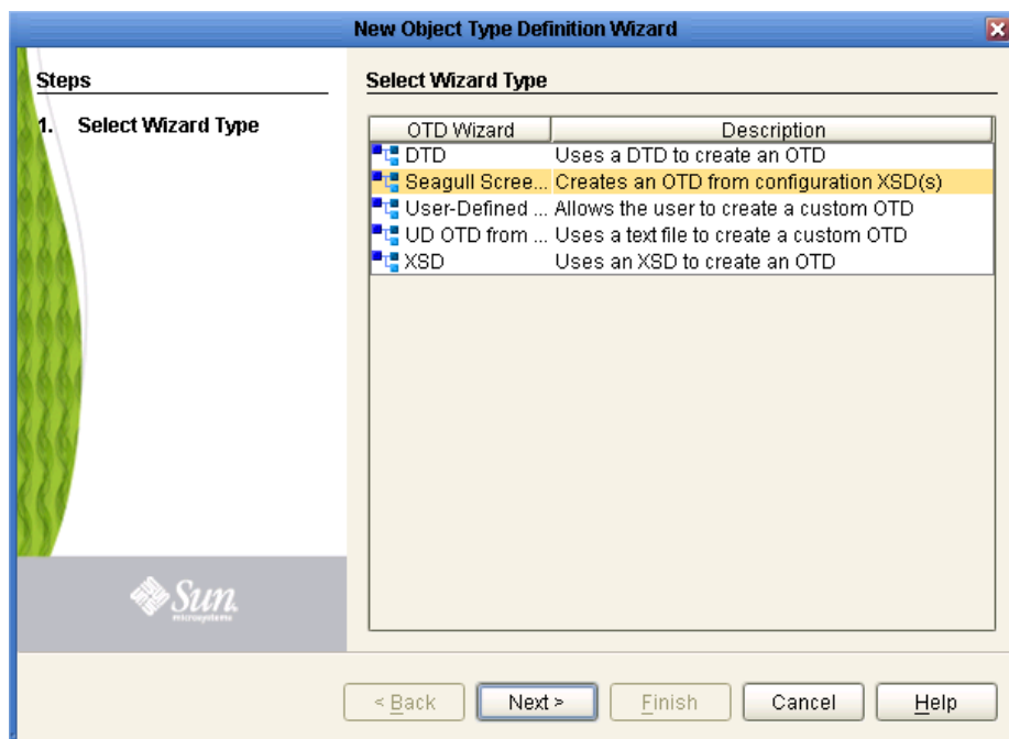
Figure 5 Select Wizard Type
