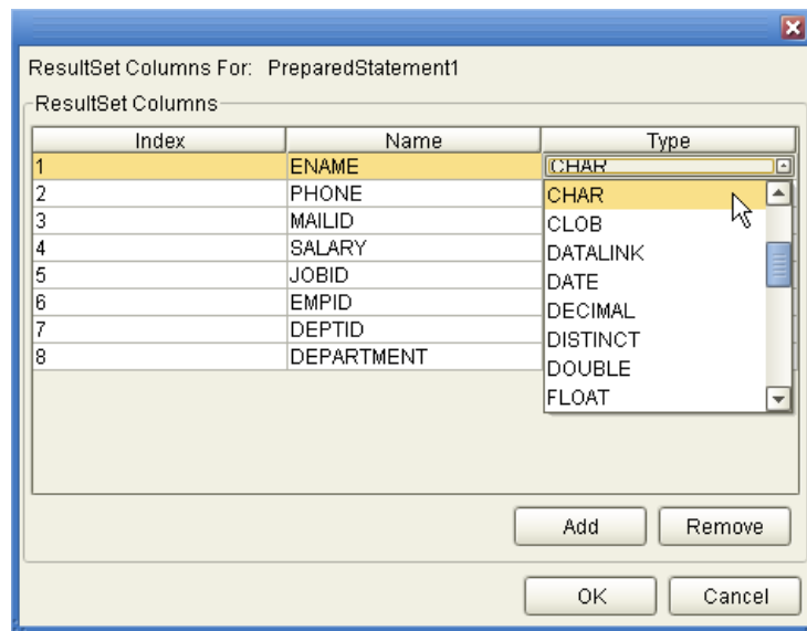
Figure 16 ResultSet Columns
