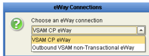
Figure 2 Template window
