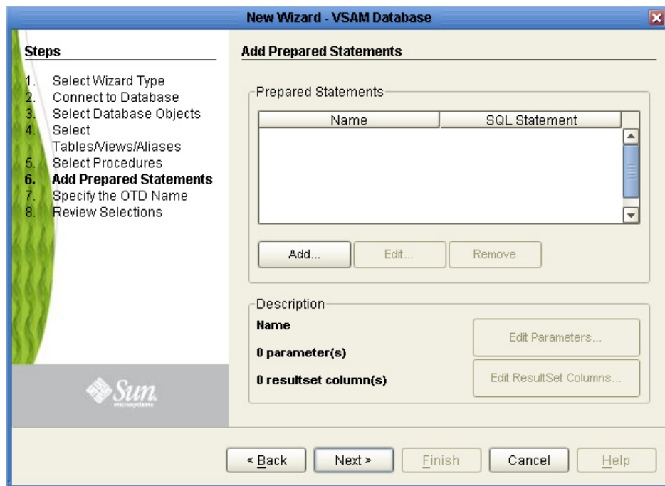
Figure 13 Prepared Statement
