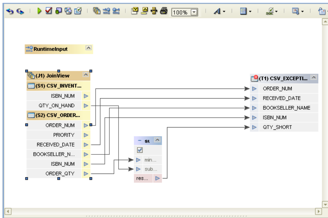
Figure 19 eTL - Graphical Views of Tables
