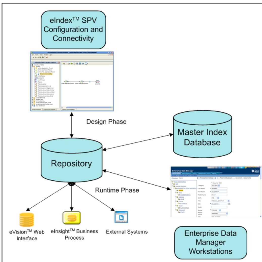
Figure 16 eIndex SPV Architecture
