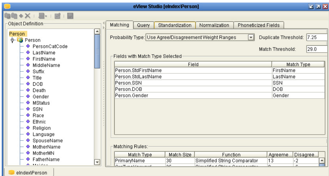
Figure 17 eIndex SPV Configuration Editor
