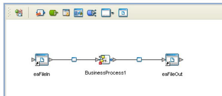
Figure 6 SWIFT eInsight Sample Project - Connectivity Map
