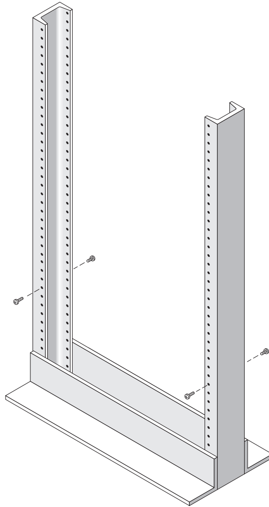
FIGURE C-2 Seating the Mounting Rails Over the Front and Back Screws
