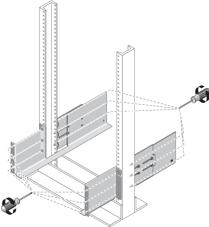
FIGURE C-4 Securing Each Rail to its Post
