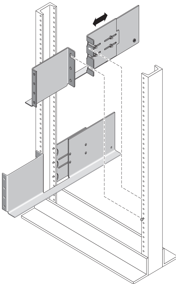
FIGURE C-2 Seating the Mounting Rails Over the Front and Back Screws
