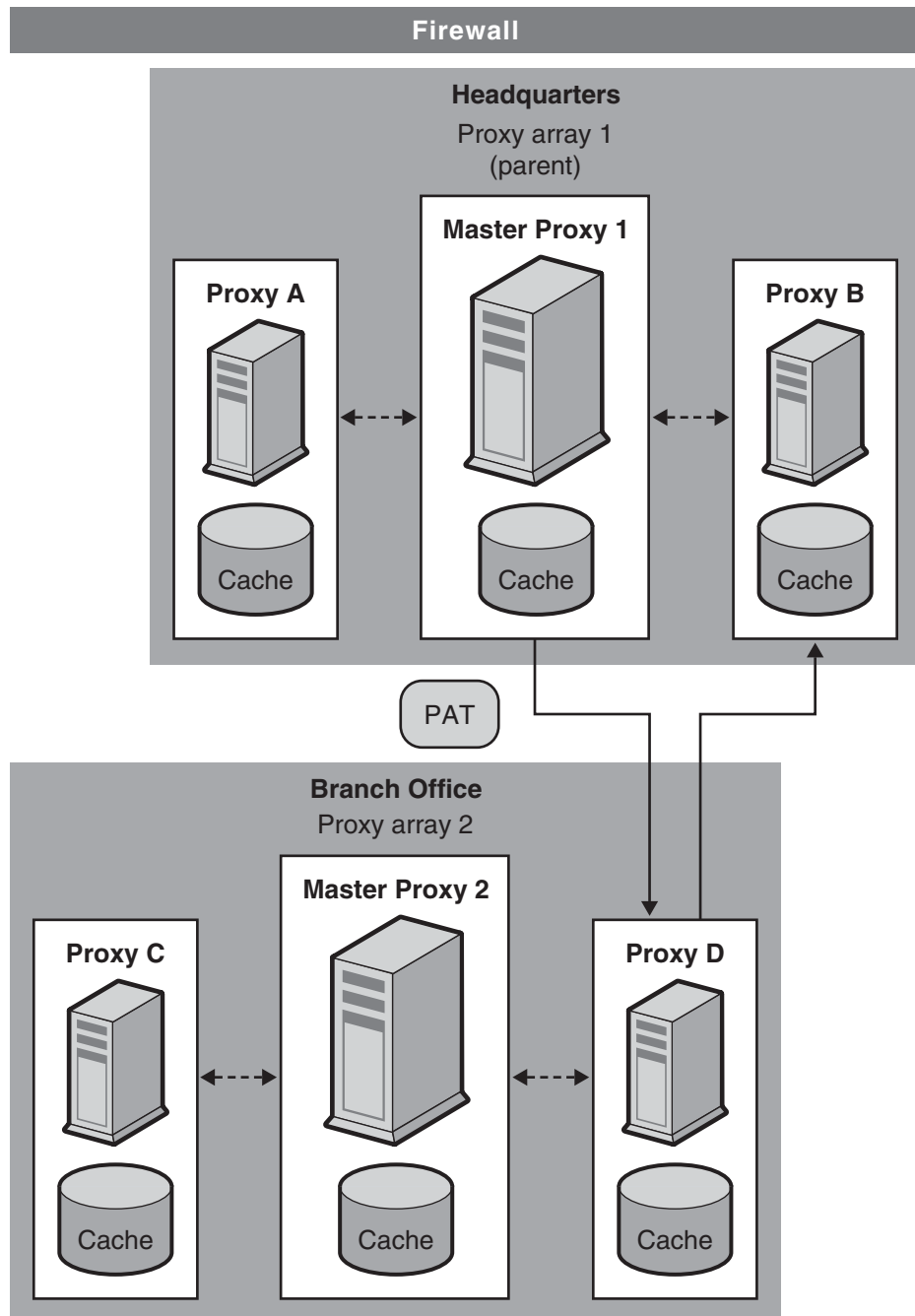
FIGURE 12-5 Proxy-to-Proxy Routing
