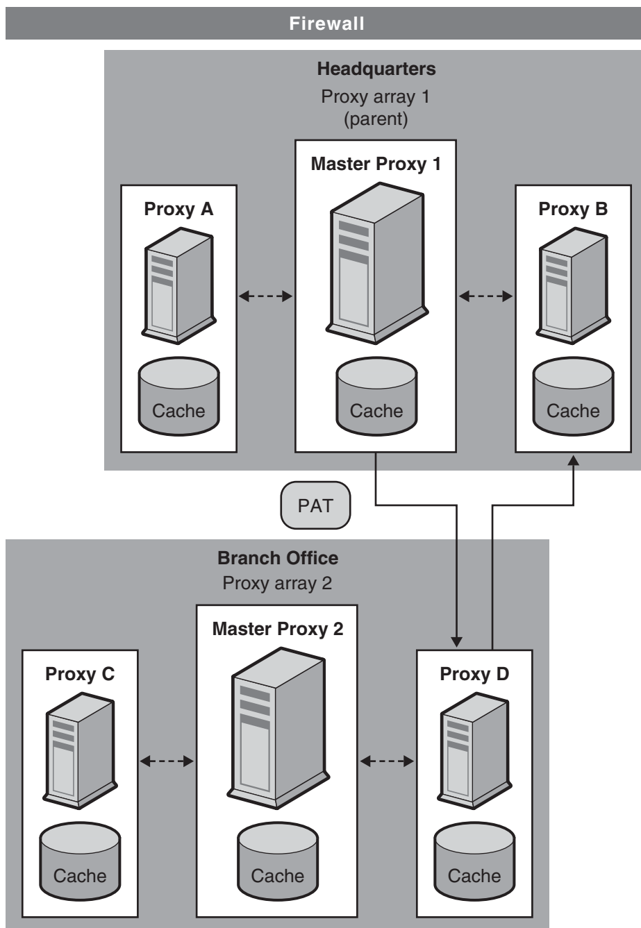
FIGURE 12-5 Proxy-to-Proxy Routing
