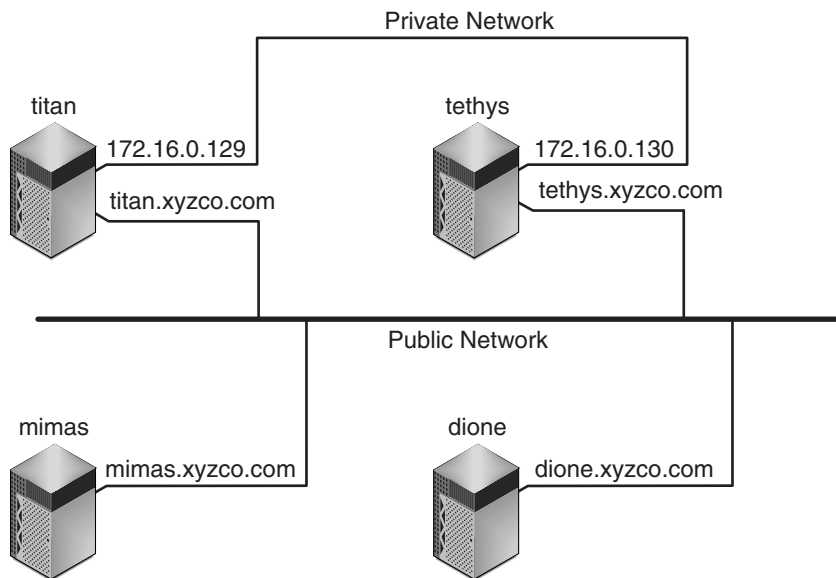
FIGURE 2-2 Network Interfaces
