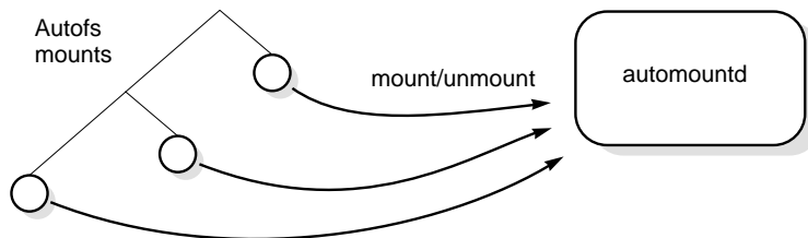
Figure 31-1 /etc/init.d/autofs Script Starts automount
