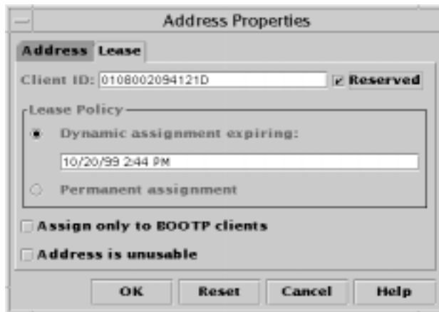
Figure 11-13 Address Properties Lease Tab
