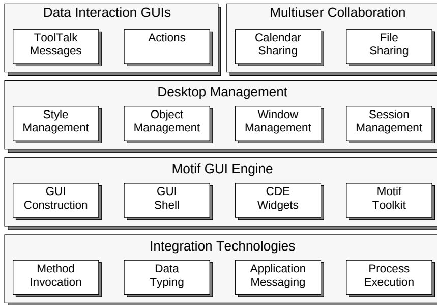
Figure 1-1 Conceptual overview of Common Desktop Environment
