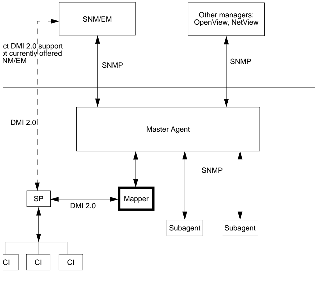
Figure 6-1 snmpXdmid Overview
