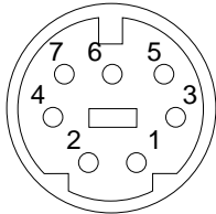
FIGURE 8-3 Expert3D Stereo Connector
