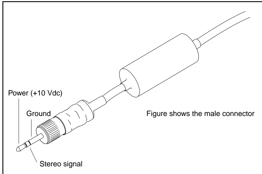
FIGURE 2-1 Creator Series 1 Stereo Connector
