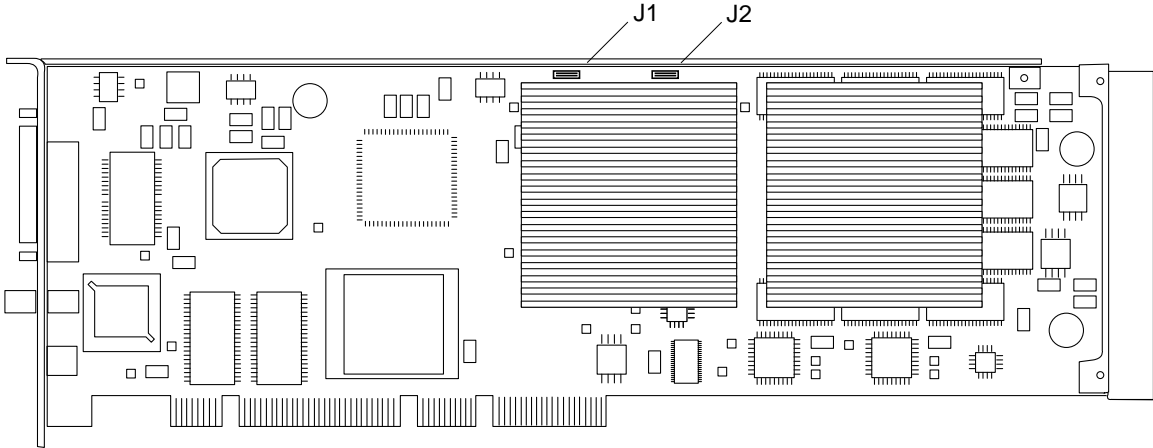
FIGURE 8-5 Expert3D Multiview In and Multiview Out Connectors
