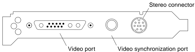
FIGURE 8-1 Expert3D External I/O Port Connectors
