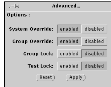
OPEN LOOK
