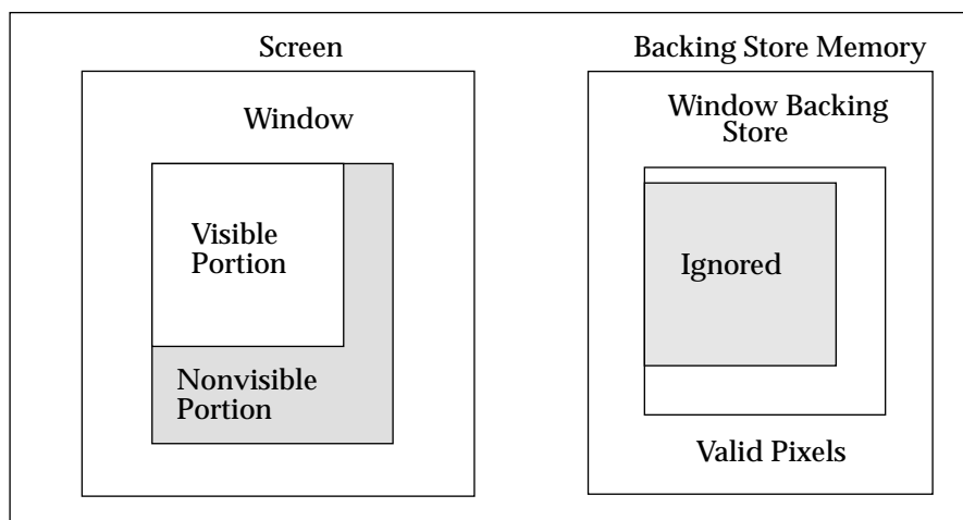
Figure 10-1 Screen and Backing Store Memory Relationship
