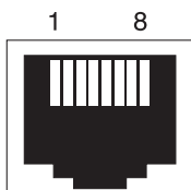
FIGURE E-1 Socket RJ-45 Ethernet 10/100 BASE-T
