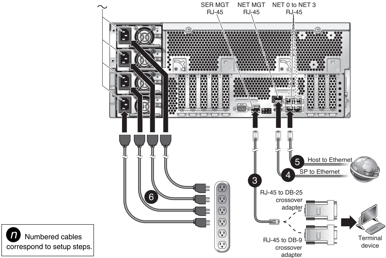
FIGURE 2 Server Connections
