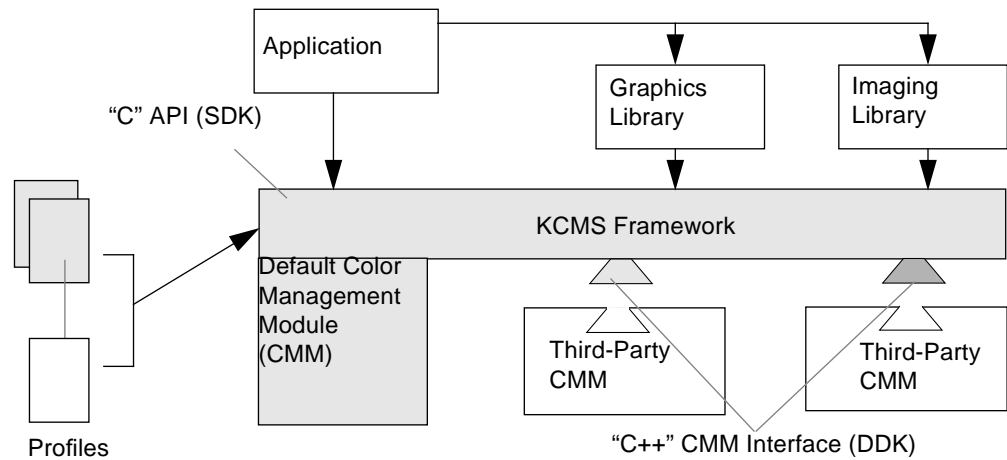
Figure 1-1 KCMS Architecture
