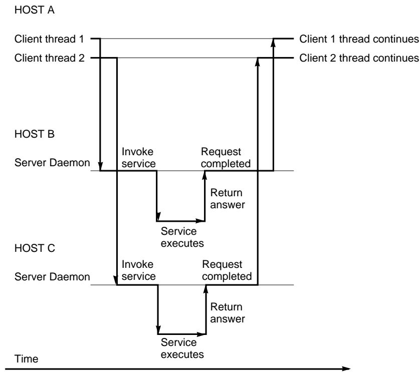
Figure 4-1 Two Client Threads Using Different Client Handles (Real time)
