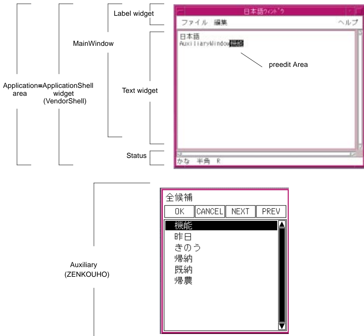
Figure 1-3 Example of VendorShell widget with auxiliary (Japanese)
