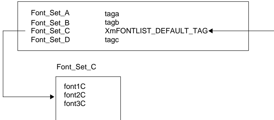
Figure 4-2 Relationships between compound strings, font sets, and font lists when a font list element tag is set to XmFONTLIST_DEFAULT_TAG
