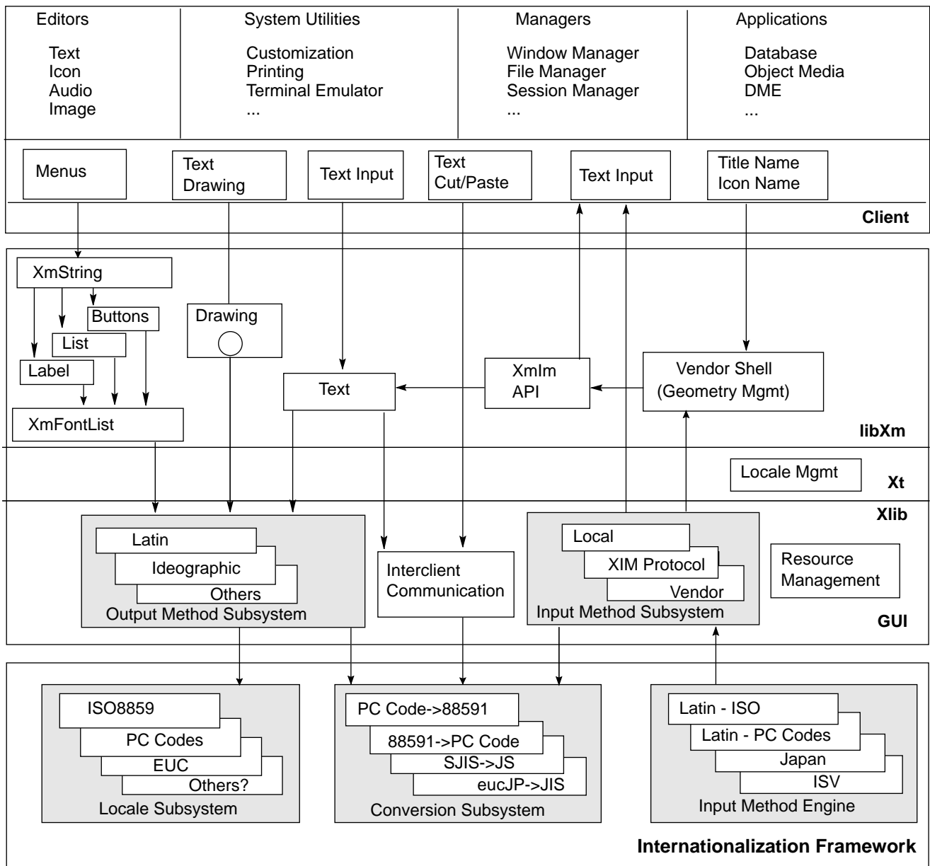
Figure 1-2 Common internationalized system
