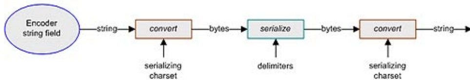
FIGURE 25 encodeToString()
