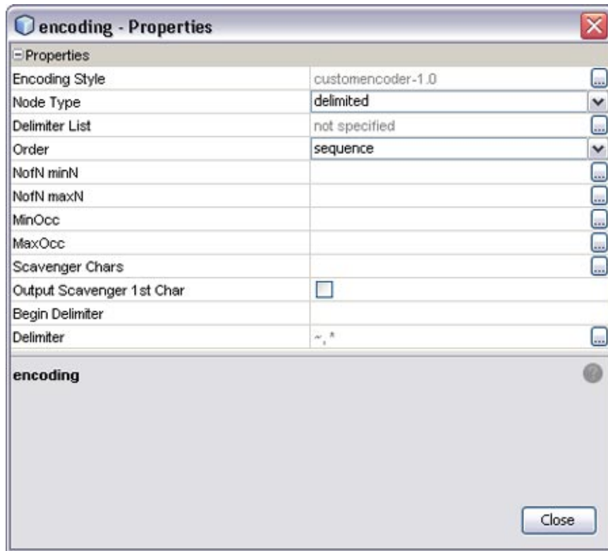
FIGURE 18 Element_2Properties
