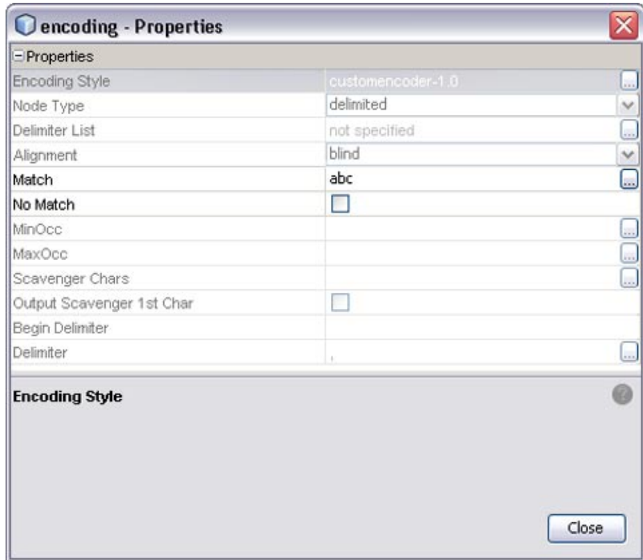
FIGURE 4 Match Property
