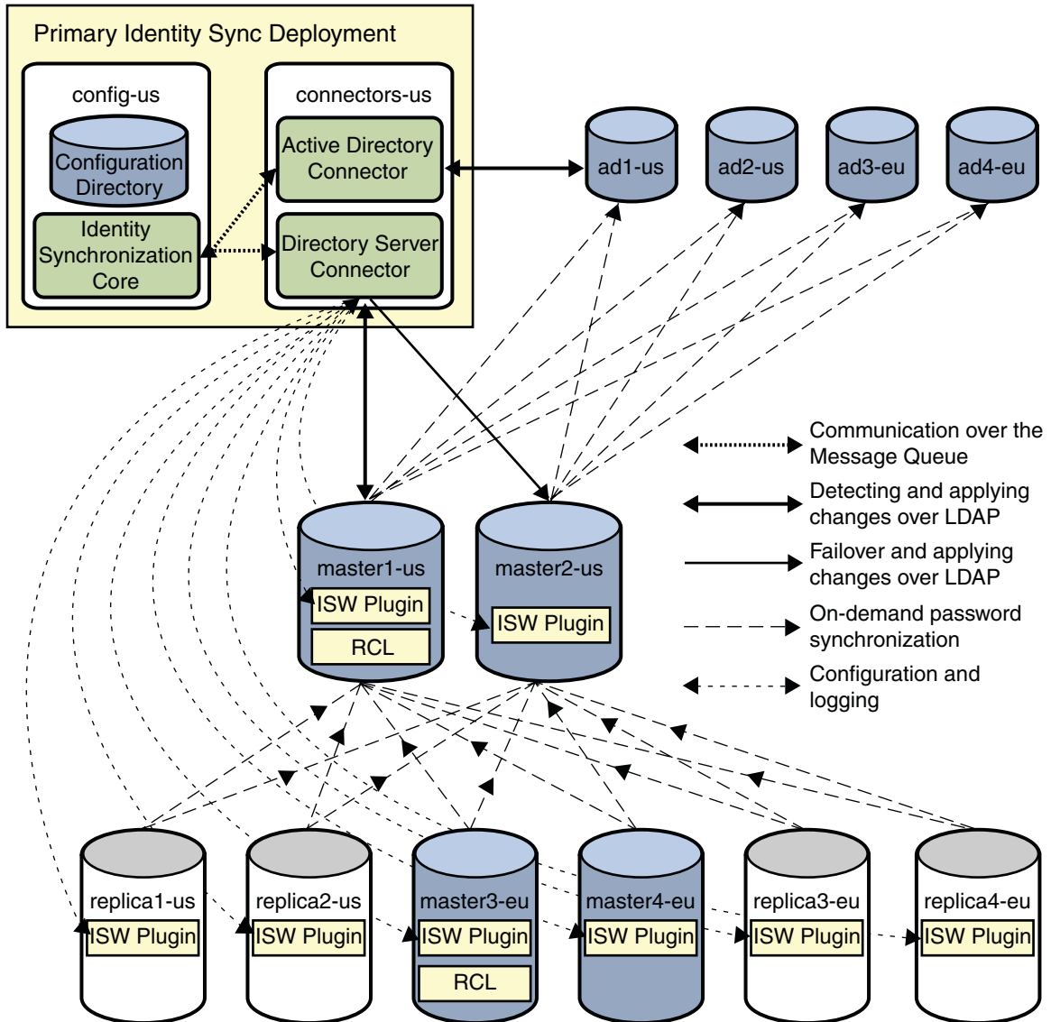
FIGURE 3-3 Primary Installation of Identity Synchronization for Windows
