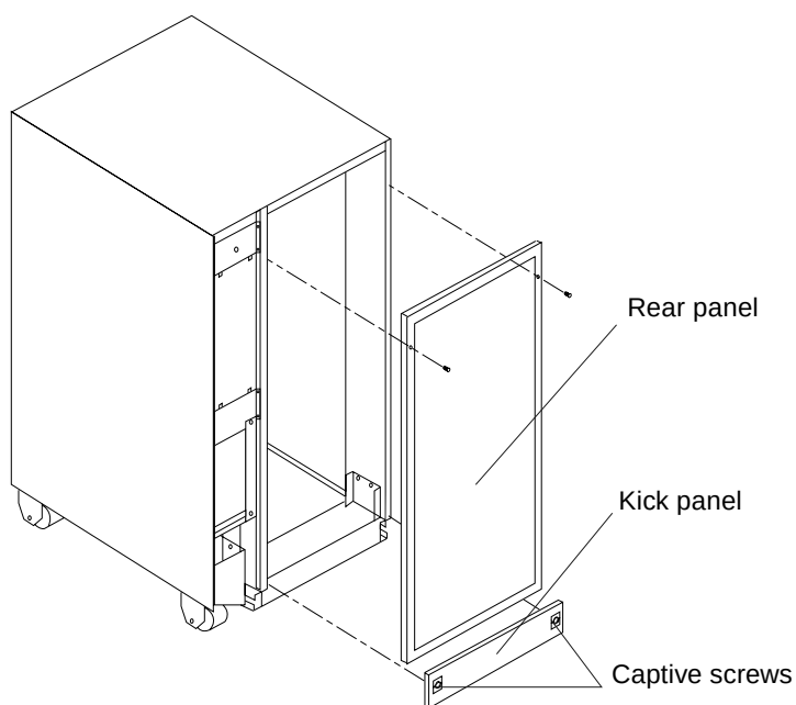
Figure 3-5 Removing the Vented Rear Panel and Kick Panel
