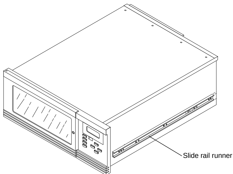
Figure 2-3 Installing Slide Rail Runners
