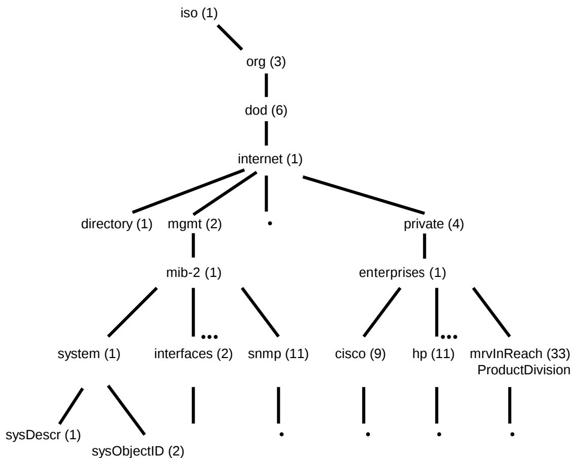
Figure 3. MIB Organization
