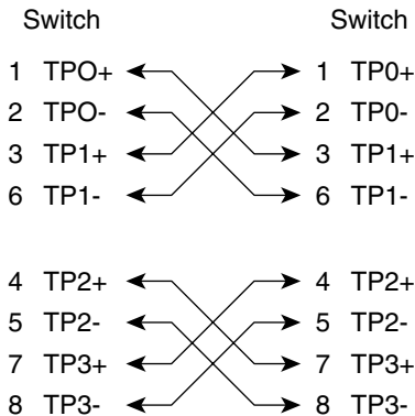
Figure B-10 Four Twisted-Pair Crossover Cable Schematics for 10/100/1000 Ports
