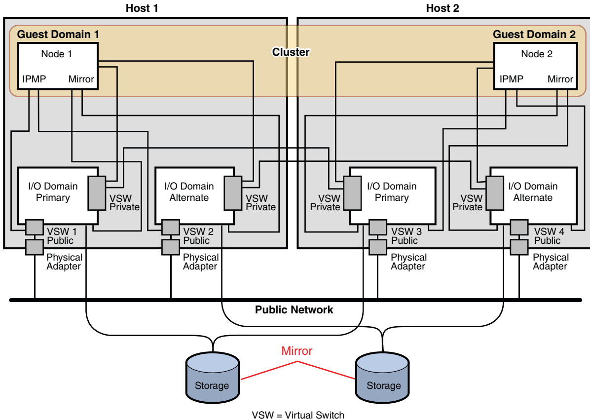
FIGURE 2-9 SPARC: Redundant I/O Domains
