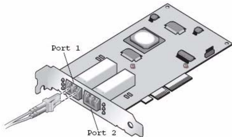
FIGURE 3 Attaching the Optical Cable
