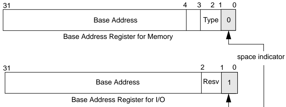
Figure 2-4 Base Address Registers for Memory and I/O
