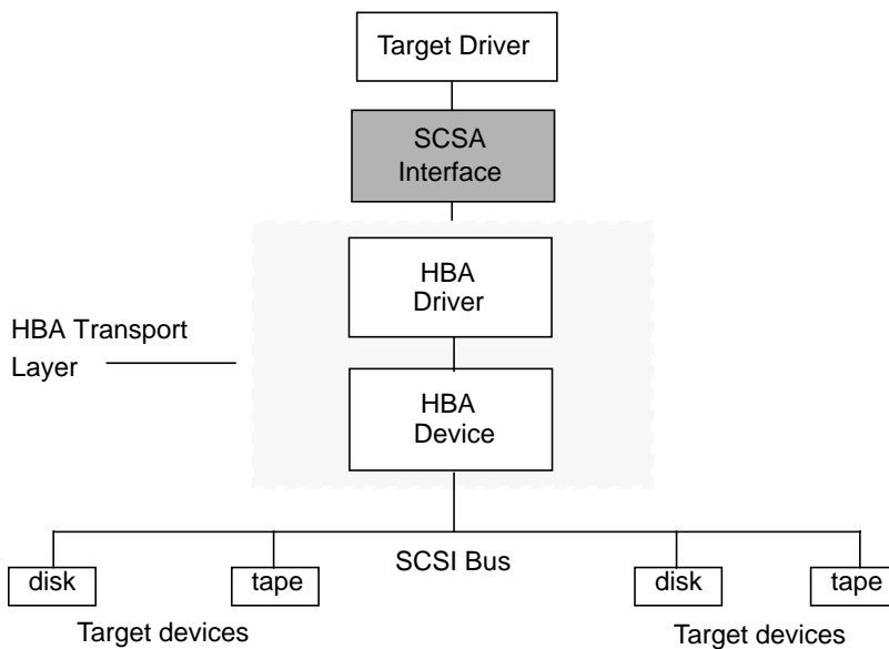
Figure 14-1 SCSA Interface
