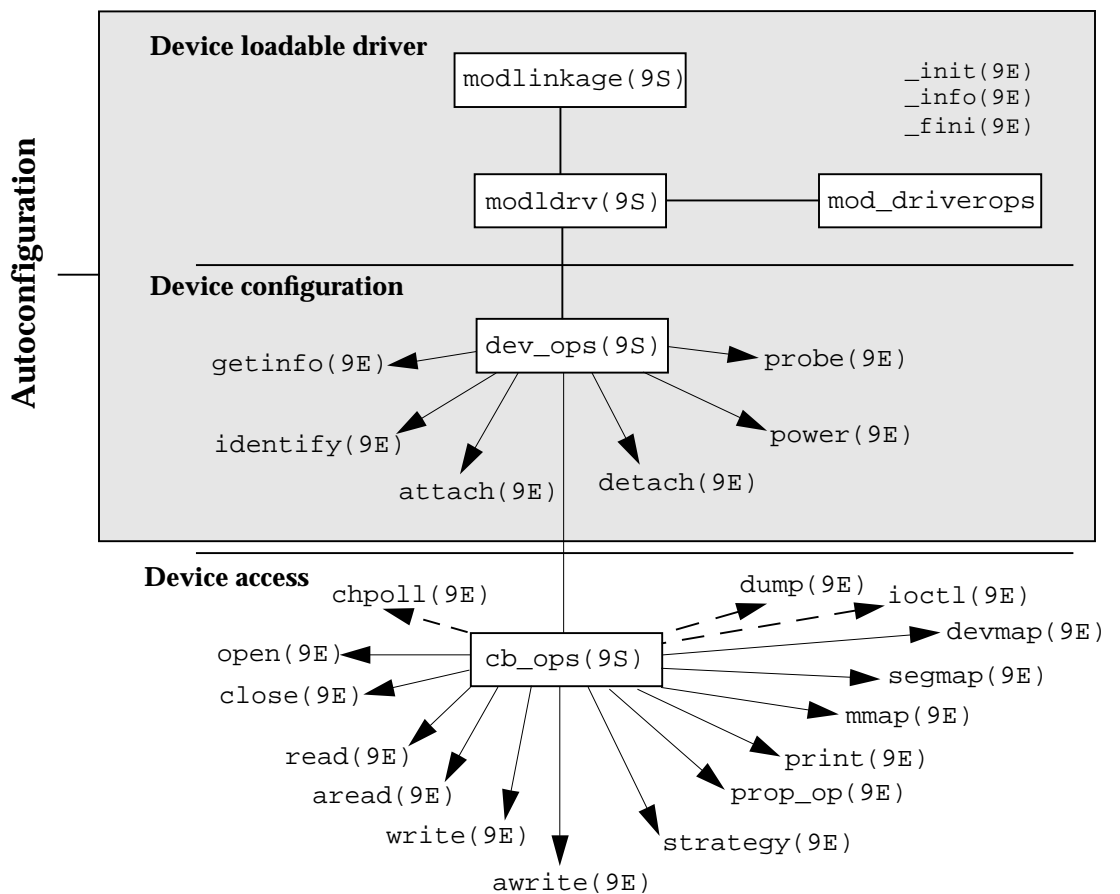
Figure 5-1 Autoconfiguration Roadmap
