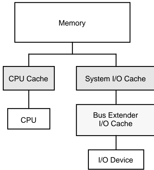
Figure 7-1 CPU and System I/O Caches
