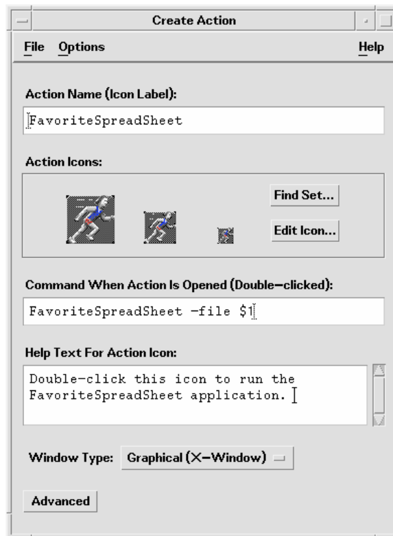
Figure 6-6 Create Action Window
