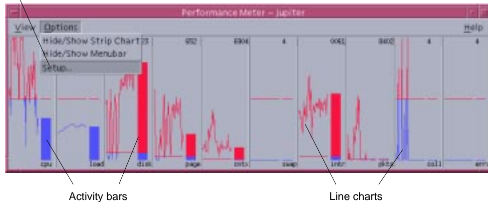
Figure 18-1 Performance Meter Displaying All Parameters (Horizontally), With Line Charts
