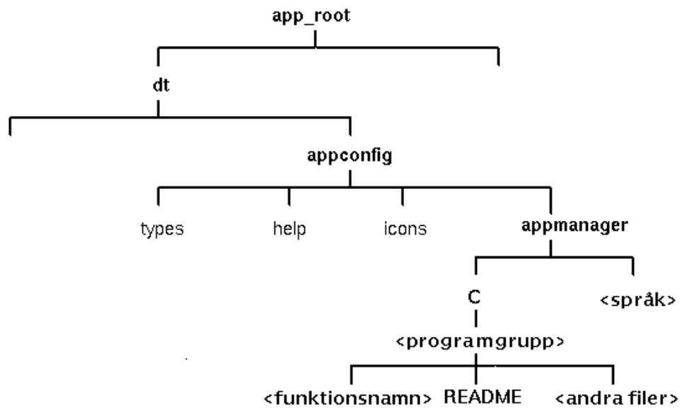
Figur 5-7 Katalogen appmanager
