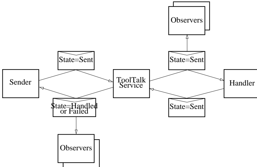
Figure 8-2 Request Routing
