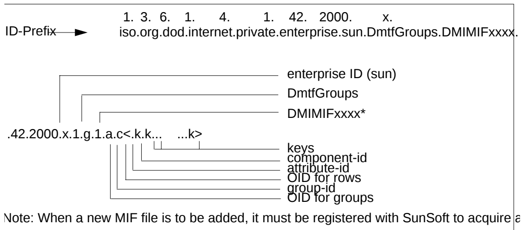
Figure 6-3 MIB OID Layout
