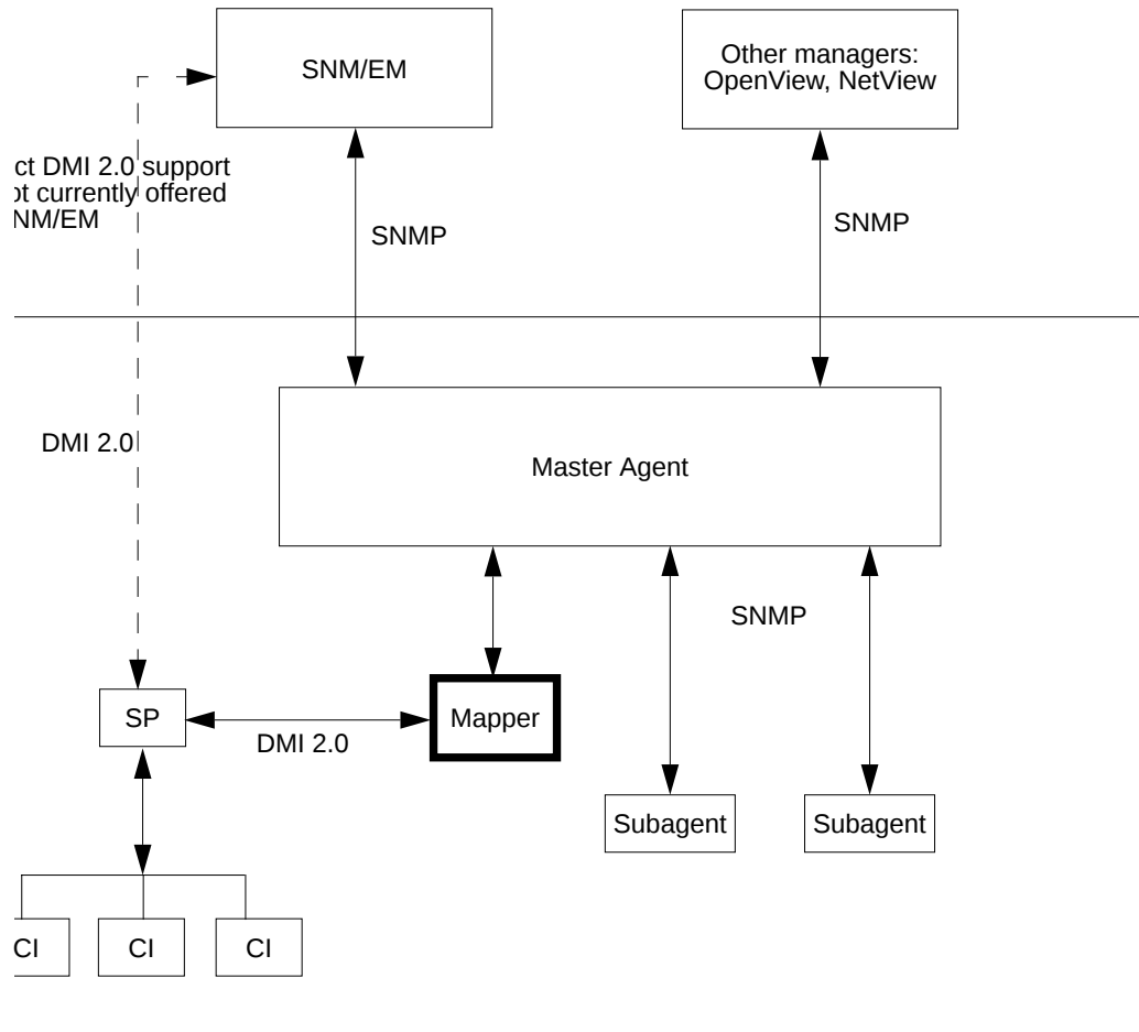
Figure 6-1 snmpXdmid Overview
