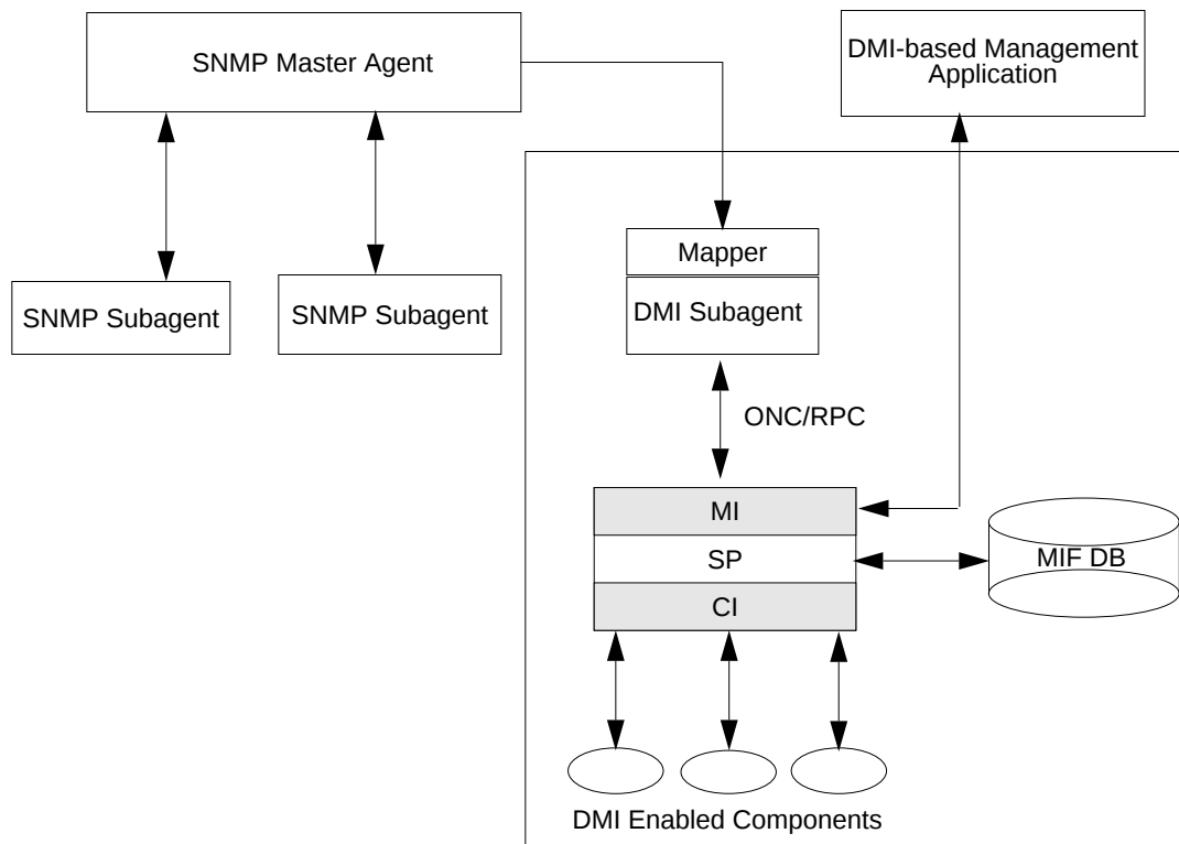
Figure 1–1 Architecture of the SEA
