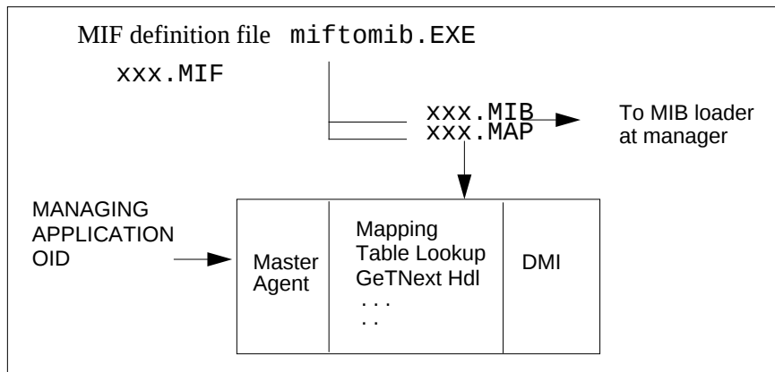
Figure 6-2 MIF-to-MIB Mapping
