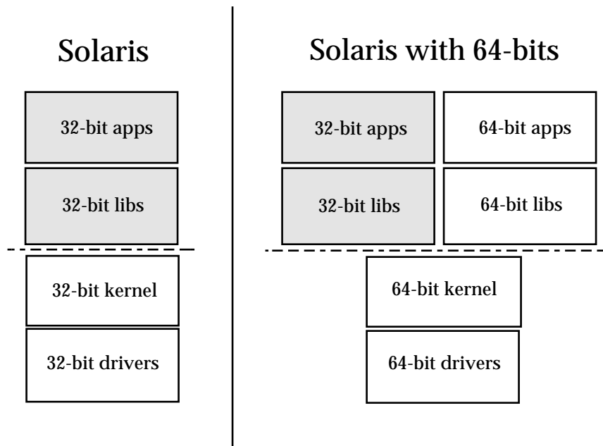
Figure 2-1 Architecture of the Solaris 7 Operating Environment
