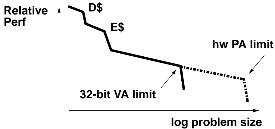
Figure 1-1 Typical Performance versus Problem Size Curve
