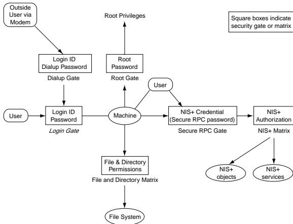
Figure 6-1 Solaris Security Gates and Filters
