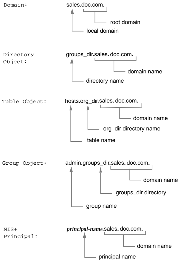
Figure 4-3 Fully qualified Names of Namespace Components
