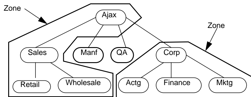
Figure 28-7 Domains and Zones
