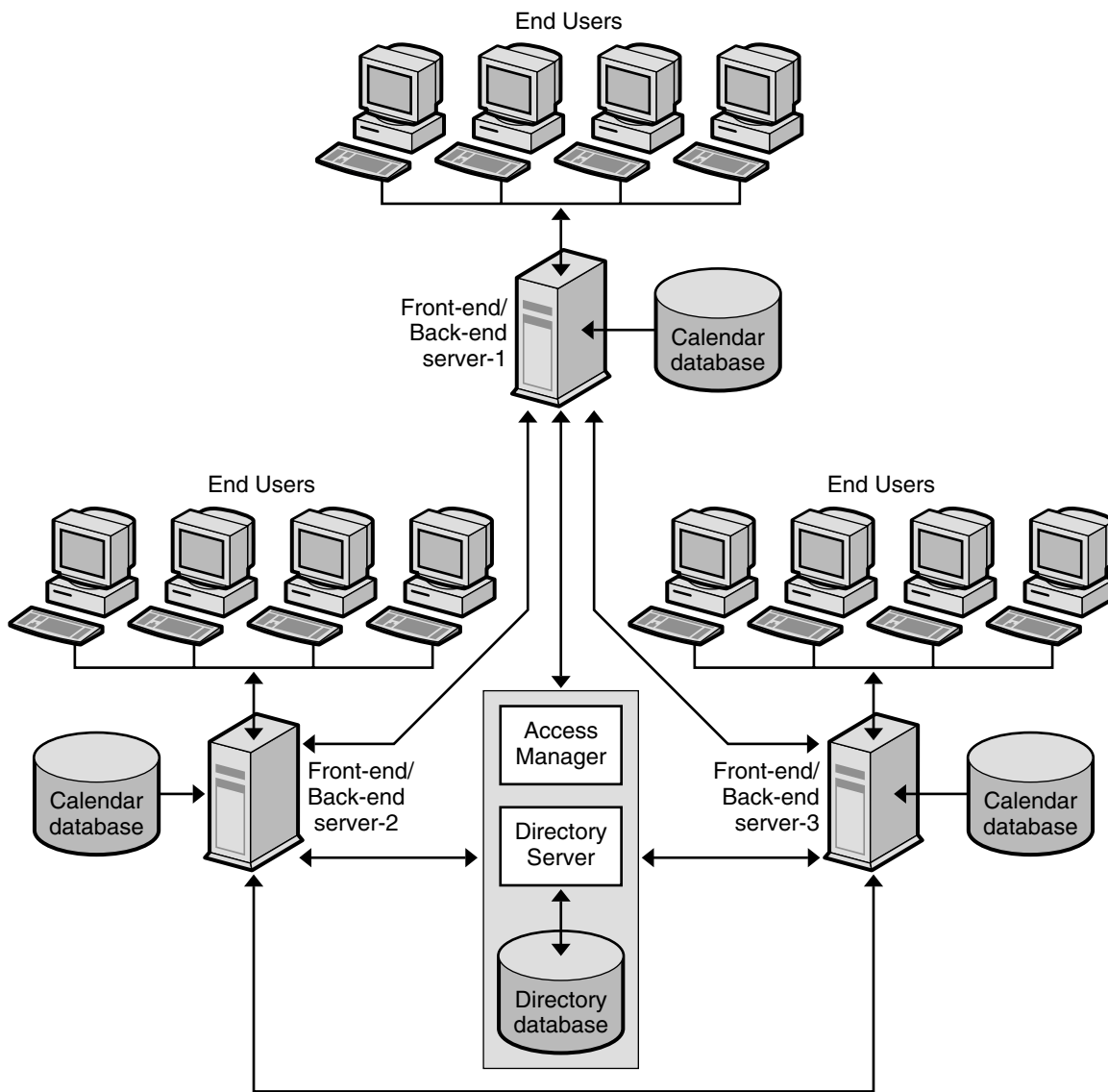
FIGURE 17-3 Two-tiered, Multiple Server Calendar Server Architecture
