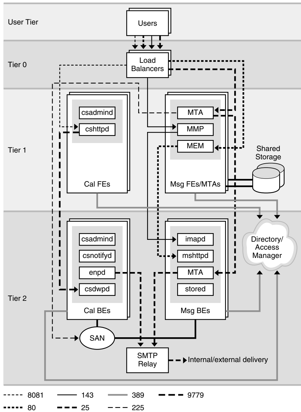
FIGURE 28-2 Communications Services Two-tiered Deployment Example
