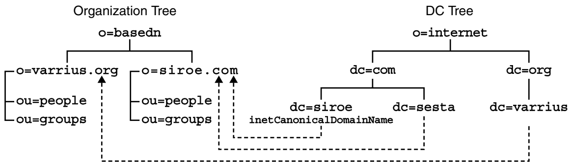
FIGURE 3-4 Two-Tree Aliasing With inetCanonicalDomainName
