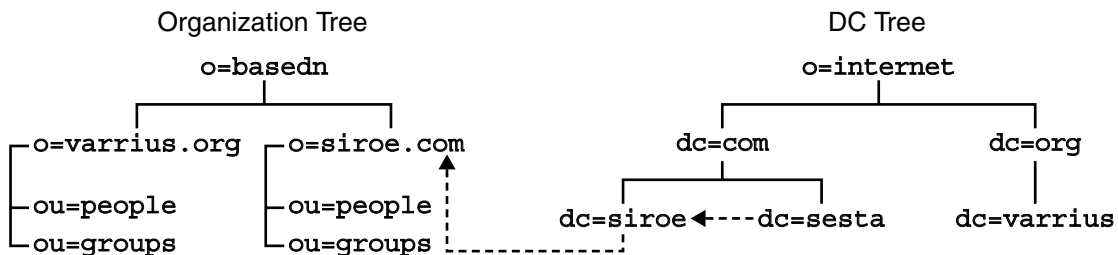
FIGURE 3-3 Two-Tree Aliasing With aliasedDomainName and inetDomainBaseDN
