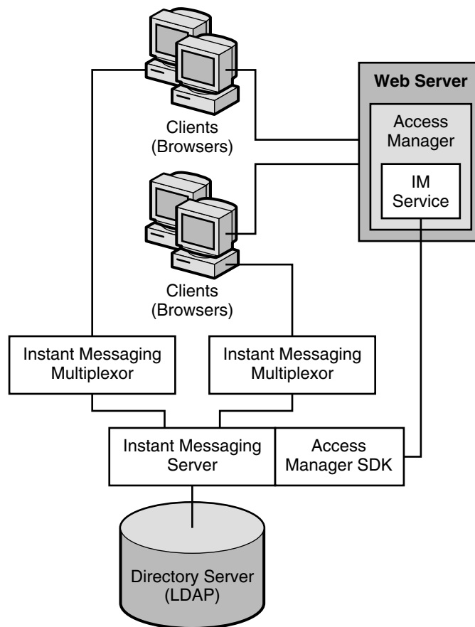
FIGURE 23-5 Instant Messaging Architecture With Access Manager-based Server Policy Management or Single Sign On
