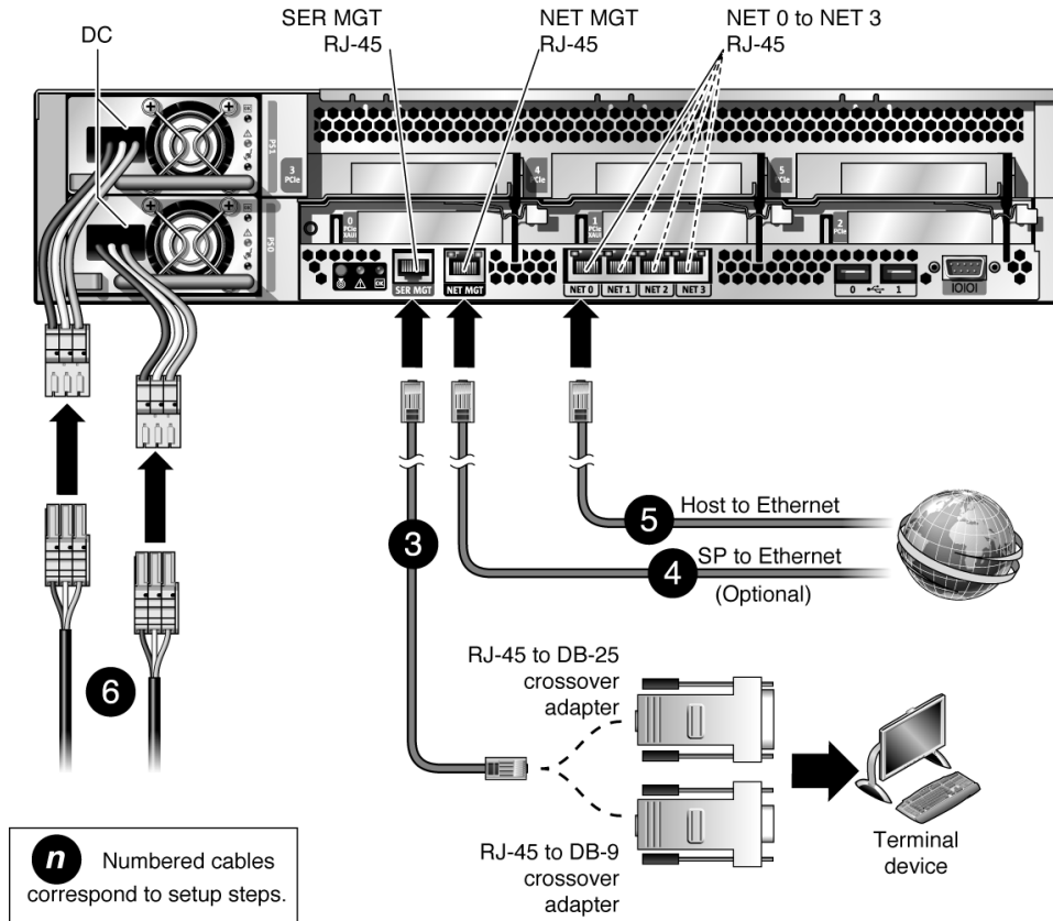
FIGURE 2 Server Connections
