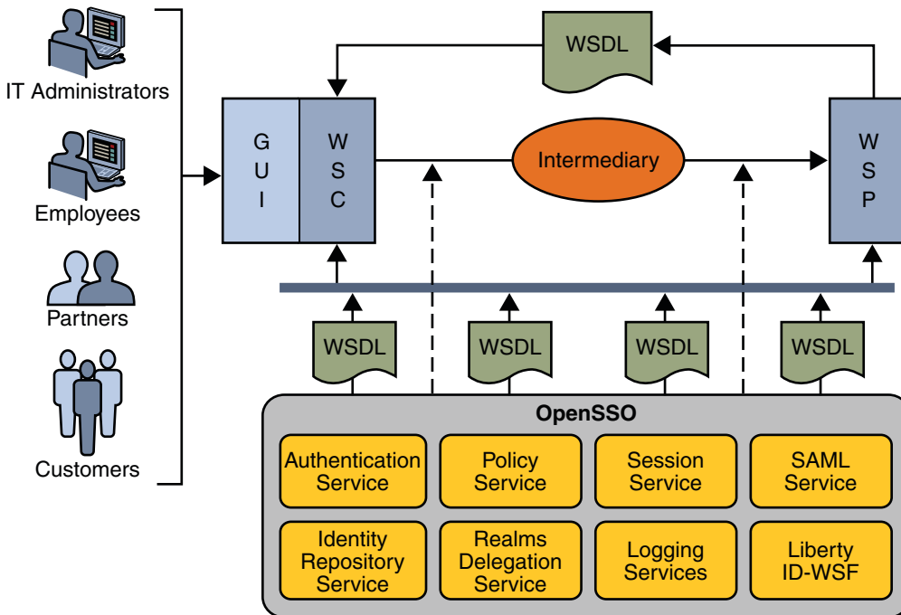
FIGURE 13-1 Components within the Identity Services Interactions
