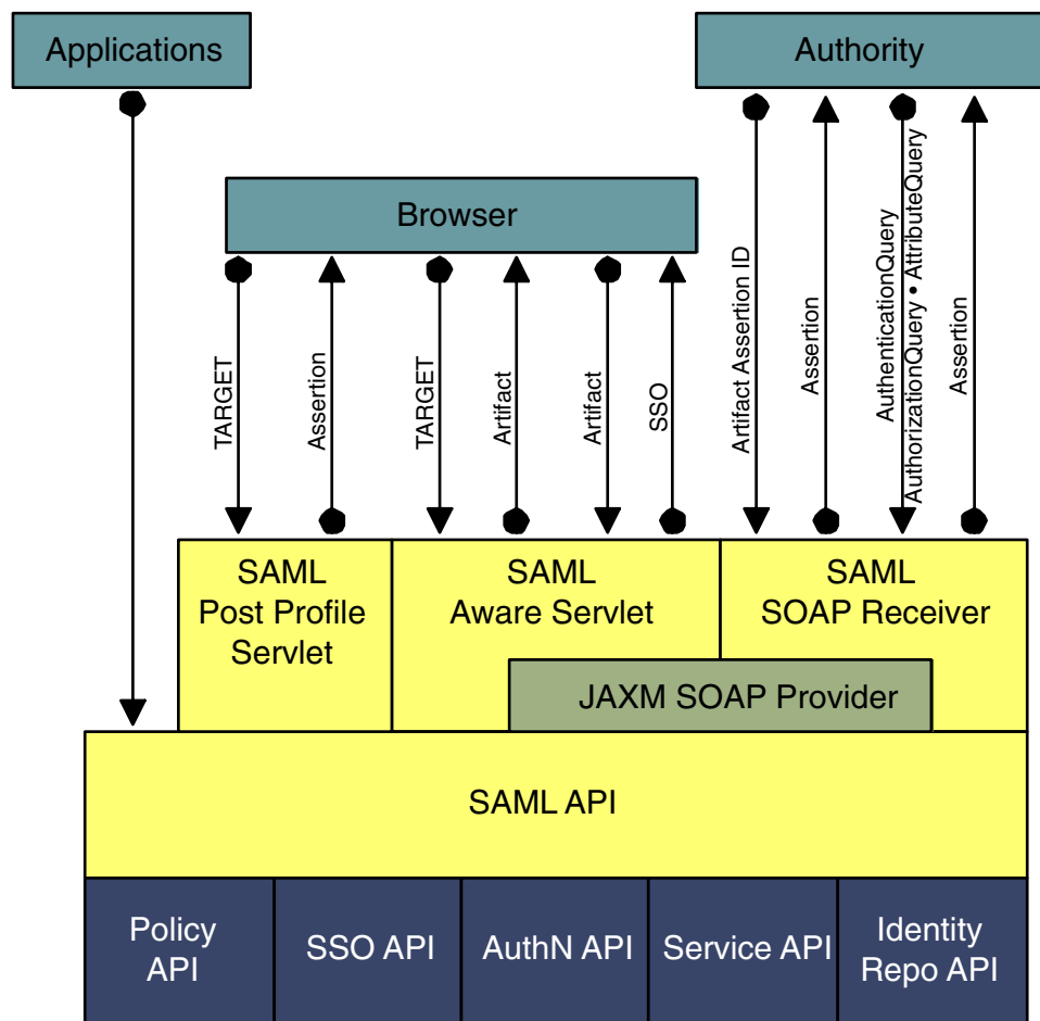
FIGURE 11–4 SAML v1.x Interaction in OpenSSO Enterprise
