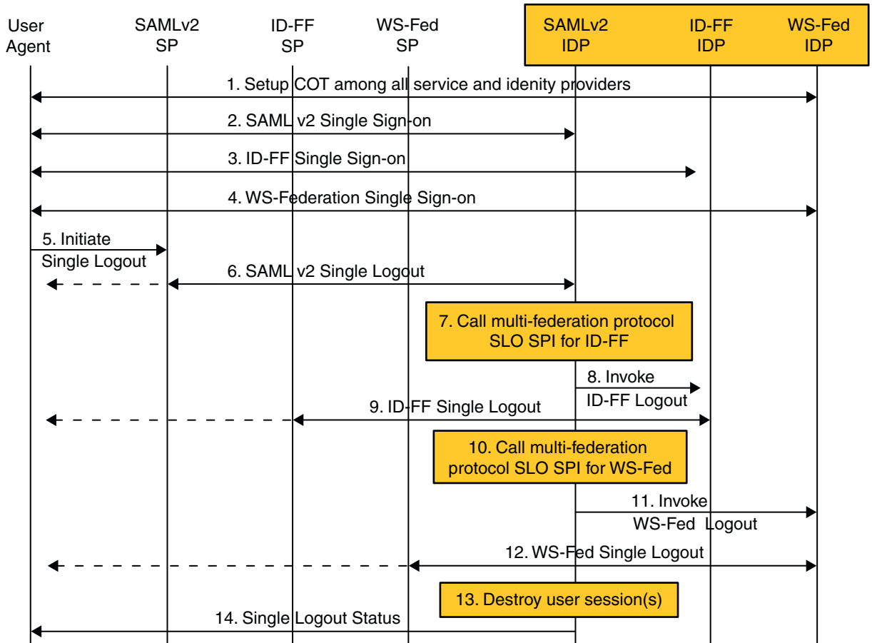
FIGURE 10–2 Multi-Federation Protocol Single Sign-on and Single Logout
