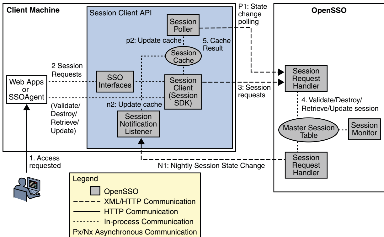
FIGURE 2-6 Session Service Components within an OpenSSO Enterprise Deployment
