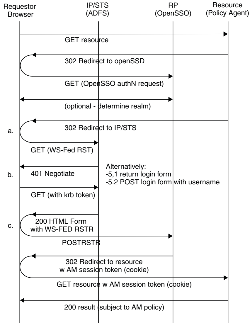
FIGURE 11-6 WS-Federation Process Flow
