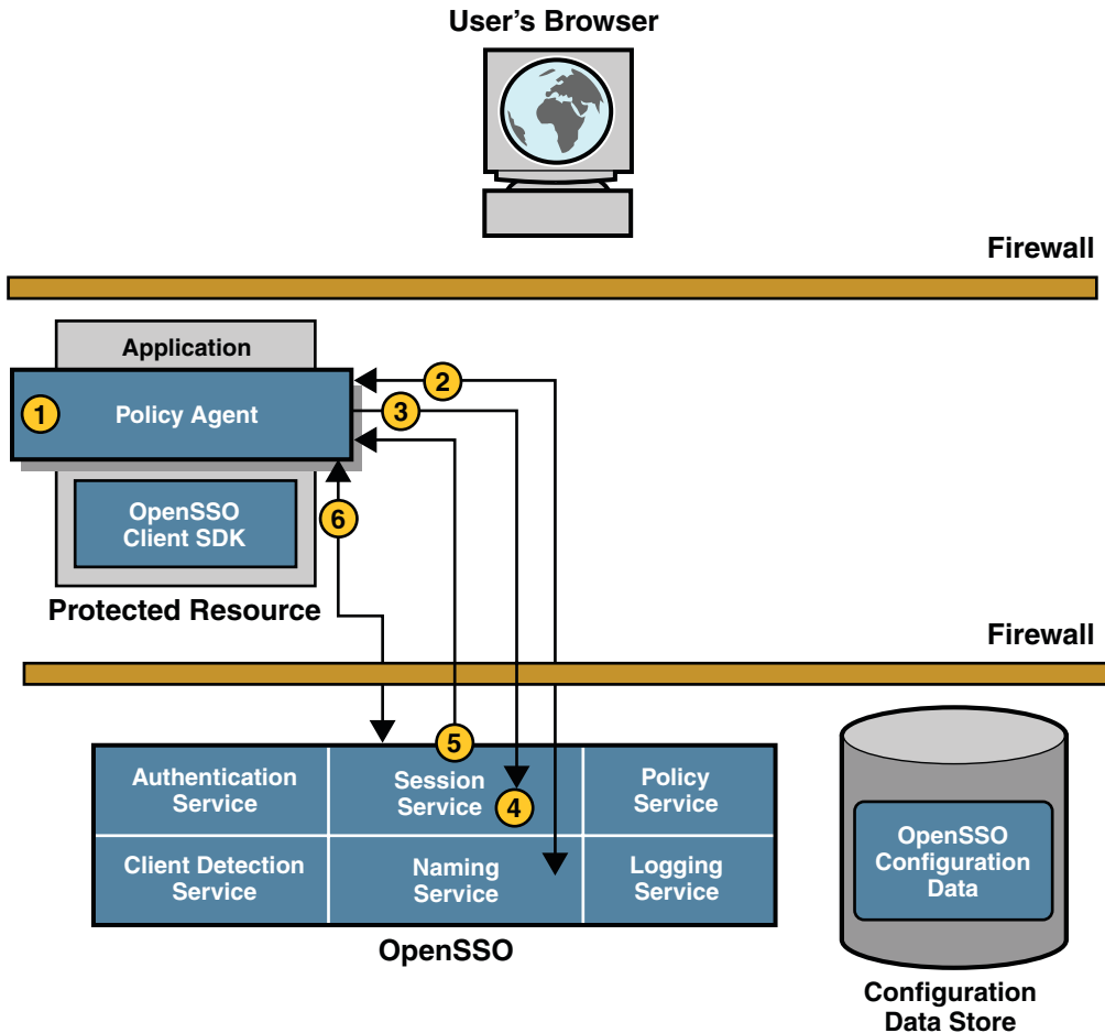
FIGURE 6-3 Session Validation
