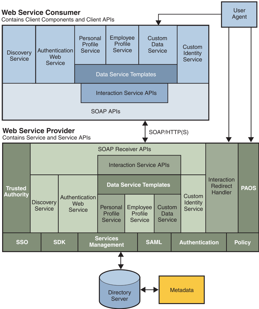
FIGURE 12-2 Web Services Stack Architecture
