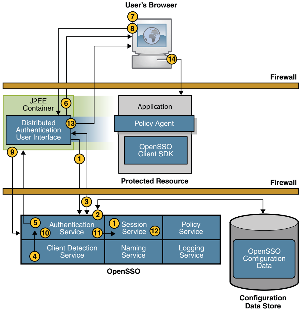
FIGURE 6-2 User Authentication
