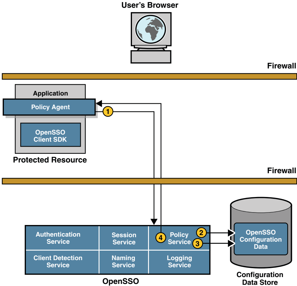
FIGURE 6-4 Policy Evaluation
