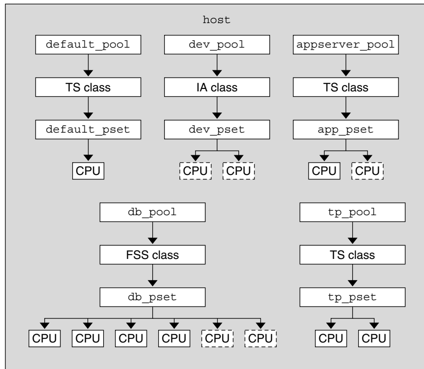
FIGURE 11-1 Server Consolidation Configuration
