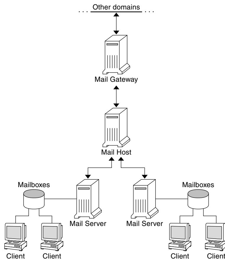
FIGURE 24-1 Typical Electronic Mail Configuration
