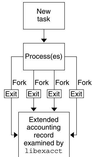
FIGURE 7-1 Task Tracking With Extended Accounting Activated
