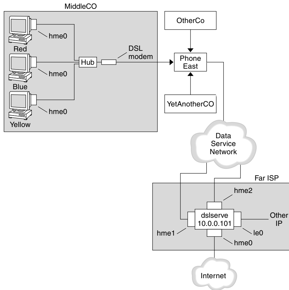
FIGURE 30-5 Example—PPPoE Tunnel
