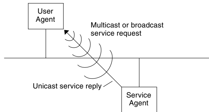
FIGURE 18-1 SLP Basic Agents and Processes
