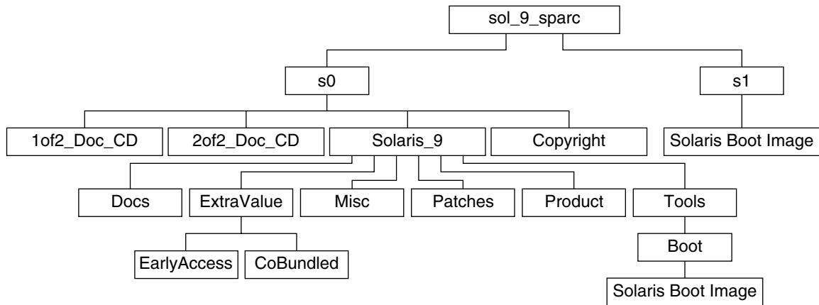
图形 38-1 Solaris 9 SPARC Platform Edition DVD
