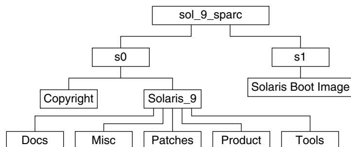
图形 38-3 SPARC : Solaris 9 Software 1 of 2 SPARC Platform Edition CD
