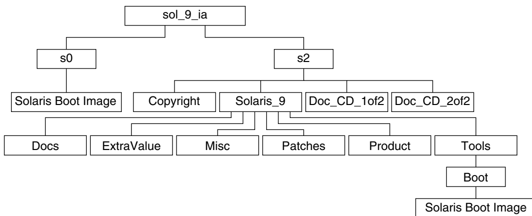
图形 38-6 Solaris 9 Intel Platform Edition DVD
