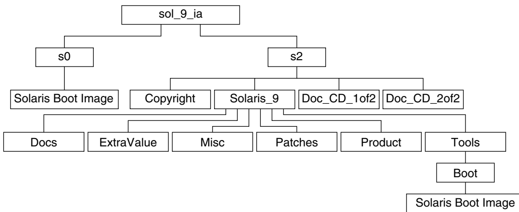
■ 38-6 Solaris 9 Intel Platform Edition DVD
