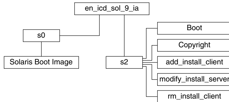
圖 38-7 IA: Solaris 9 Intel Platform Edition Installation CD
