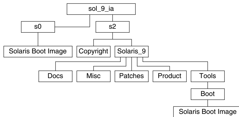
圖 38-8 IA: Solaris 9 Software 1 of 2 Intel Platform Edition CD
