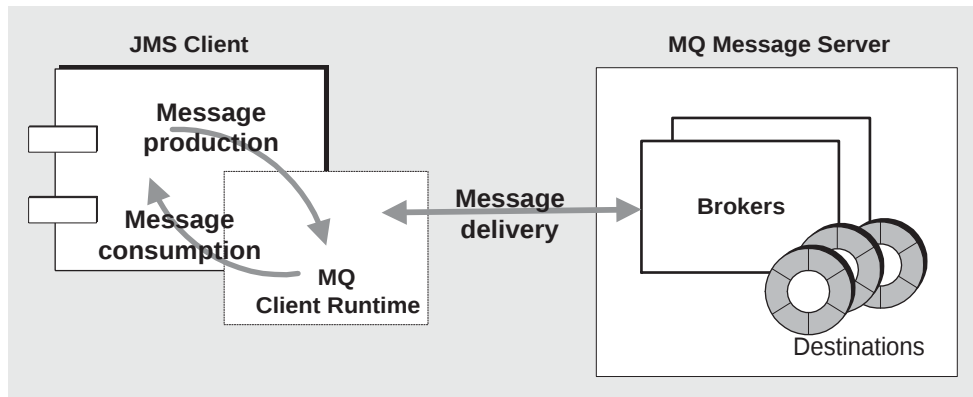
Figure 2-8 Messaging Operations
