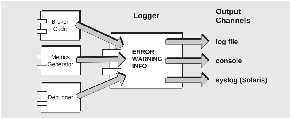
Figure 2-6 Logging Scheme
